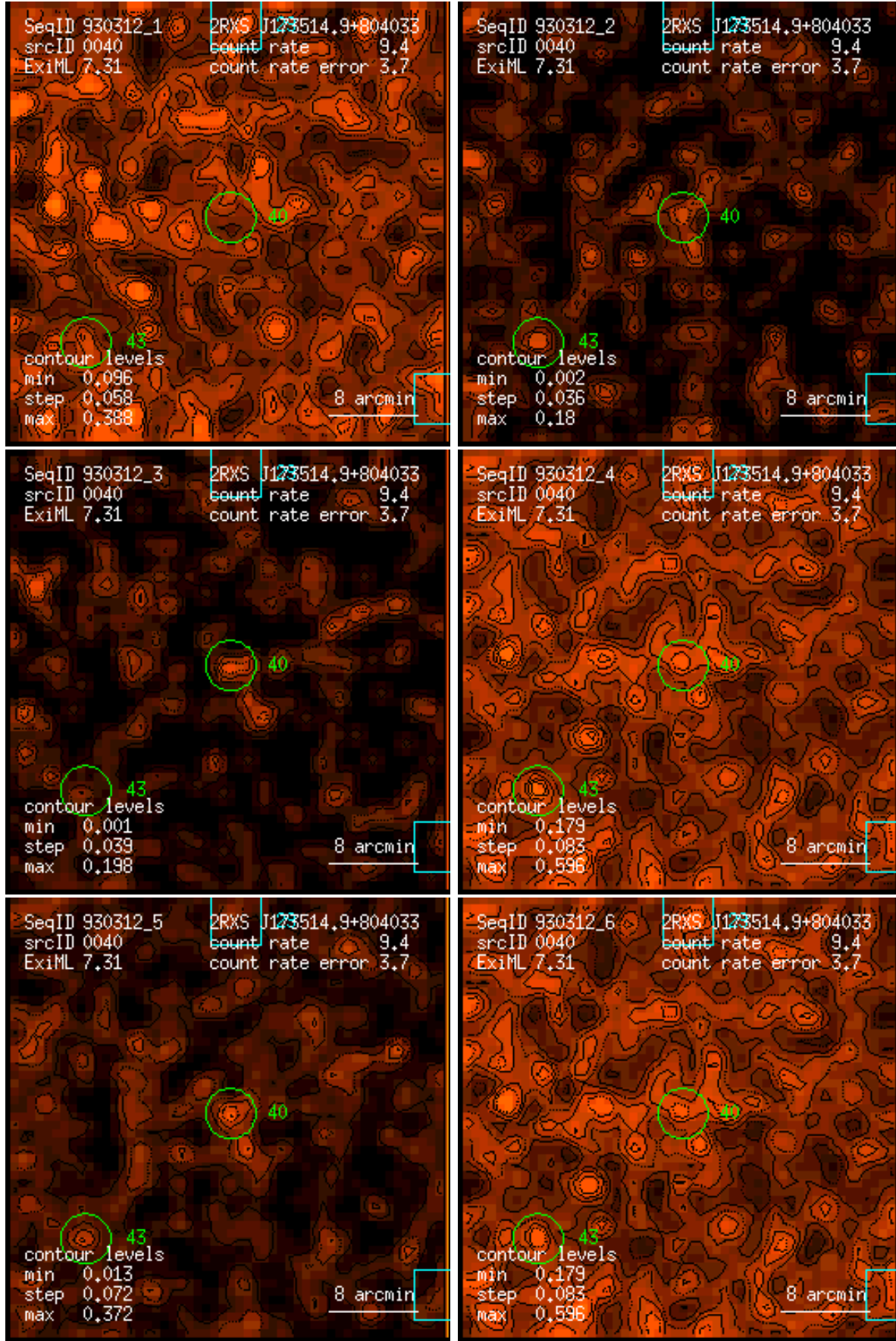
Figure 40: RASS 930312: detection 0040: band rate images, Gaussian filter: (1) PSPC channels 11 – 41, (2) 52 – 90, (3) 91 – 201, (4) 11 – 235, (5) 52 – 201, (6) 11 – 201. Broad band rates in counts/ks. Band rate contour levels in counts/ks/arcmin 2 .
