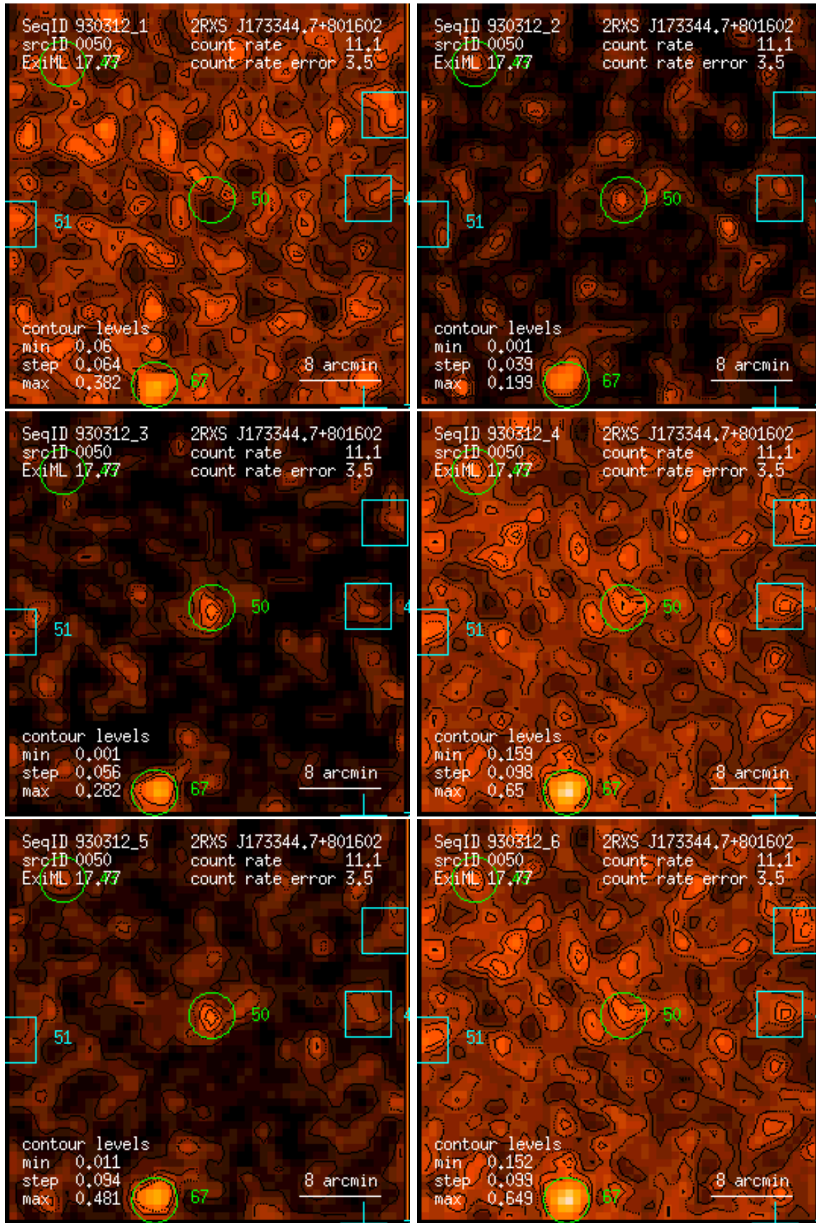
Figure 50: RASS 930312: detection 0050: band rate images, Gaussian filter: (1) PSPC channels 11 – 41, (2) 52 – 90, (3) 91 – 201, (4) 11 – 235, (5) 52 – 201, (6) 11 – 201. Broad band rates in counts/ks. Band rate contour levels in counts/ks/arcmin 2 .
