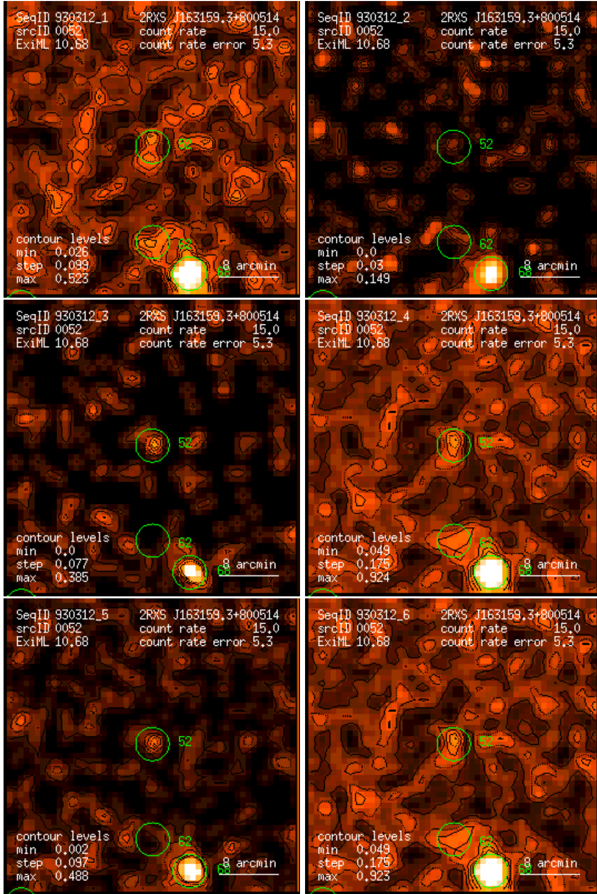
Figure 52: RASS 930312: detection 0052: band rate images, Gaussian filter: (1) PSPC channels 11 – 41, (2) 52 – 90, (3) 91 – 201, (4) 11 – 235, (5) 52 – 201, (6) 11 – 201. Broad band rates in counts/ks. Band rate contour levels in counts/ks/arcmin 2 .
