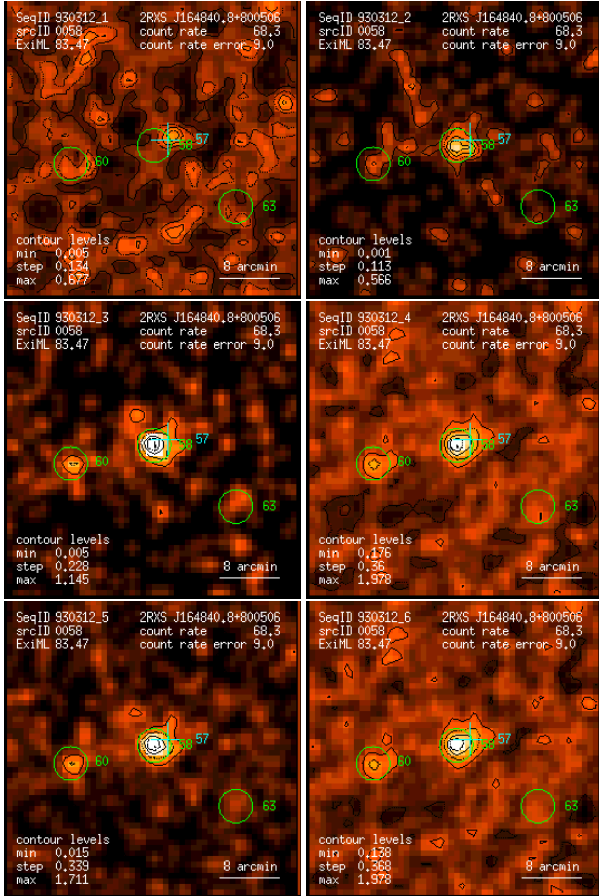
Figure 58: RASS 930312: detection 0058: band rate images, Gaussian filter: (1) PSPC channels 11 – 41, (2) 52 – 90, (3) 91 – 201, (4) 11 – 235, (5) 52 – 201, (6) 11 – 201. Broad band rates in counts/ks. Band rate contour levels in counts/ks/arcmin 2 .
