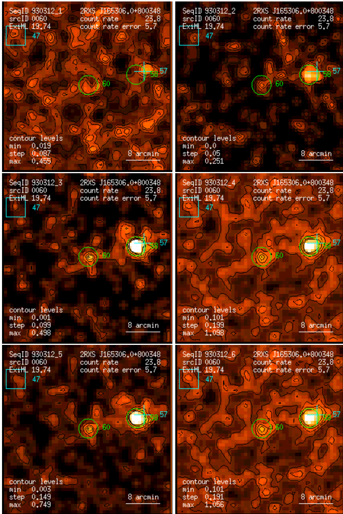
Figure 60: RASS 930312: detection 0060: band rate images, Gaussian filter: (1) PSPC channels 11 – 41, (2) 52 – 90, (3) 91 – 201, (4) 11 – 235, (5) 52 – 201, (6) 11 – 201. Broad band rates in counts/ks. Band rate contour levels in counts/ks/arcmin 2 .
