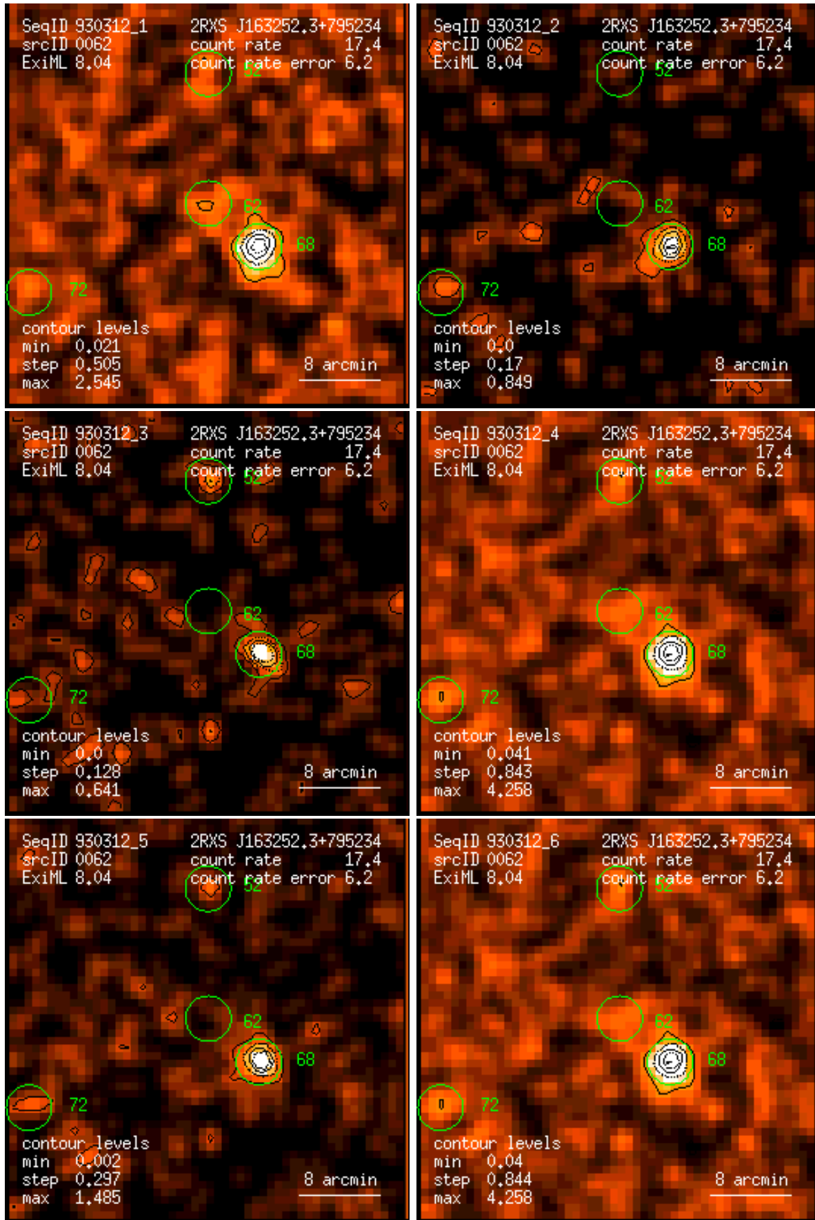
Figure 62: RASS 930312: detection 0062: band rate images, Gaussian filter: (1) PSPC channels 11 – 41, (2) 52 – 90, (3) 91 – 201, (4) 11 – 235, (5) 52 – 201, (6) 11 – 201. Broad band rates in counts/ks. Band rate contour levels in counts/ks/arcmin 2 .
