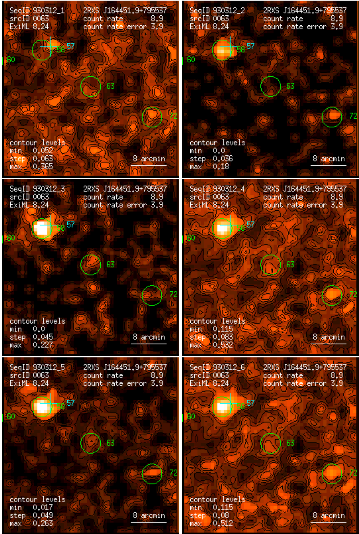
Figure 63: RASS 930312: detection 0063: band rate images, Gaussian filter: (1) PSPC channels 11 – 41, (2) 52 – 90, (3) 91 – 201, (4) 11 – 235, (5) 52 – 201, (6) 11 – 201. Broad band rates in counts/ks. Band rate contour levels in counts/ks/arcmin 2 .
