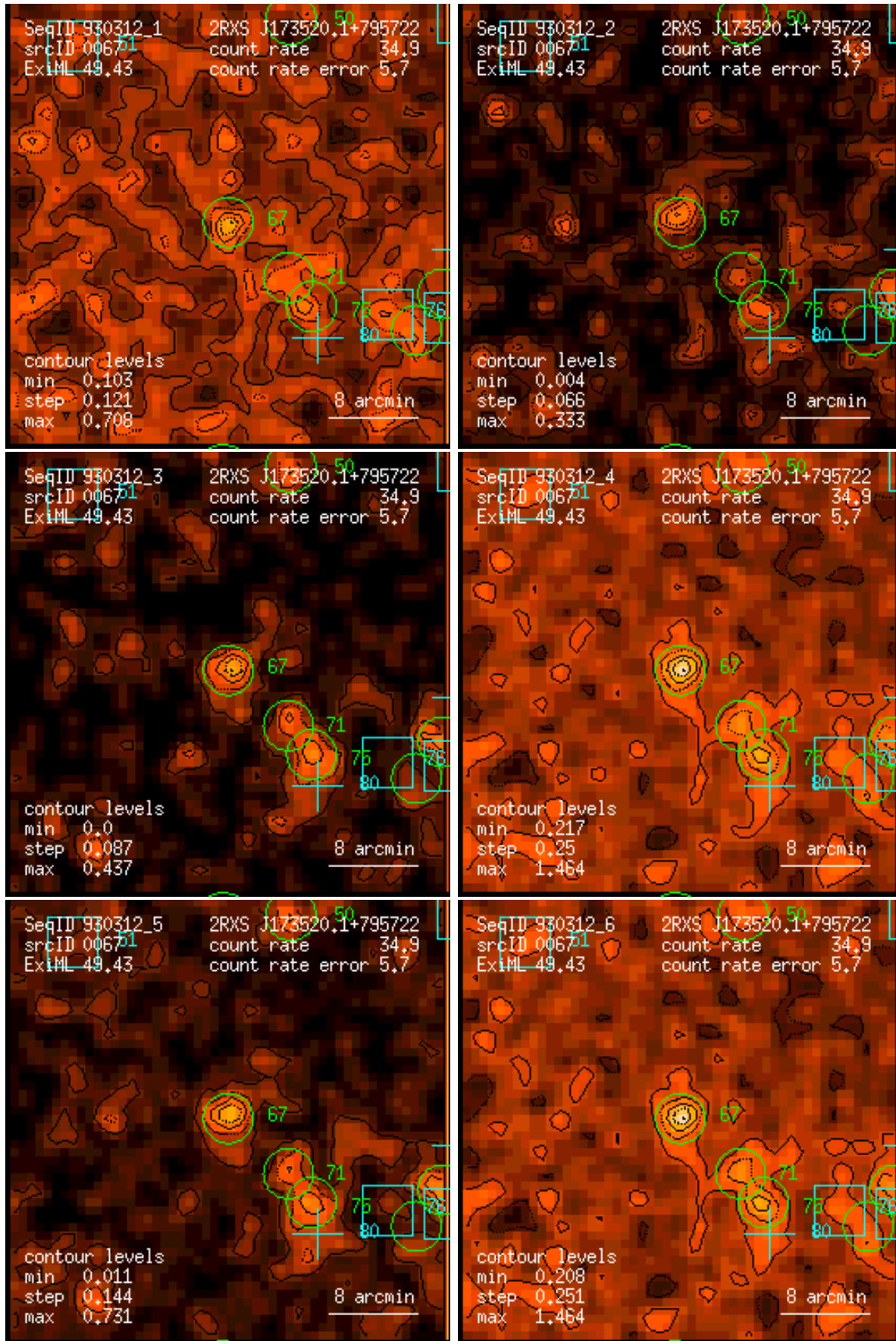
Figure 67: RASS 930312: detection 0067: band rate images, Gaussian filter: (1) PSPC channels 11 – 41, (2) 52 – 90, (3) 91 – 201, (4) 11 – 235, (5) 52 – 201, (6) 11 – 201. Broad band rates in counts/ks. Band rate contour levels in counts/ks/arcmin 2 .
