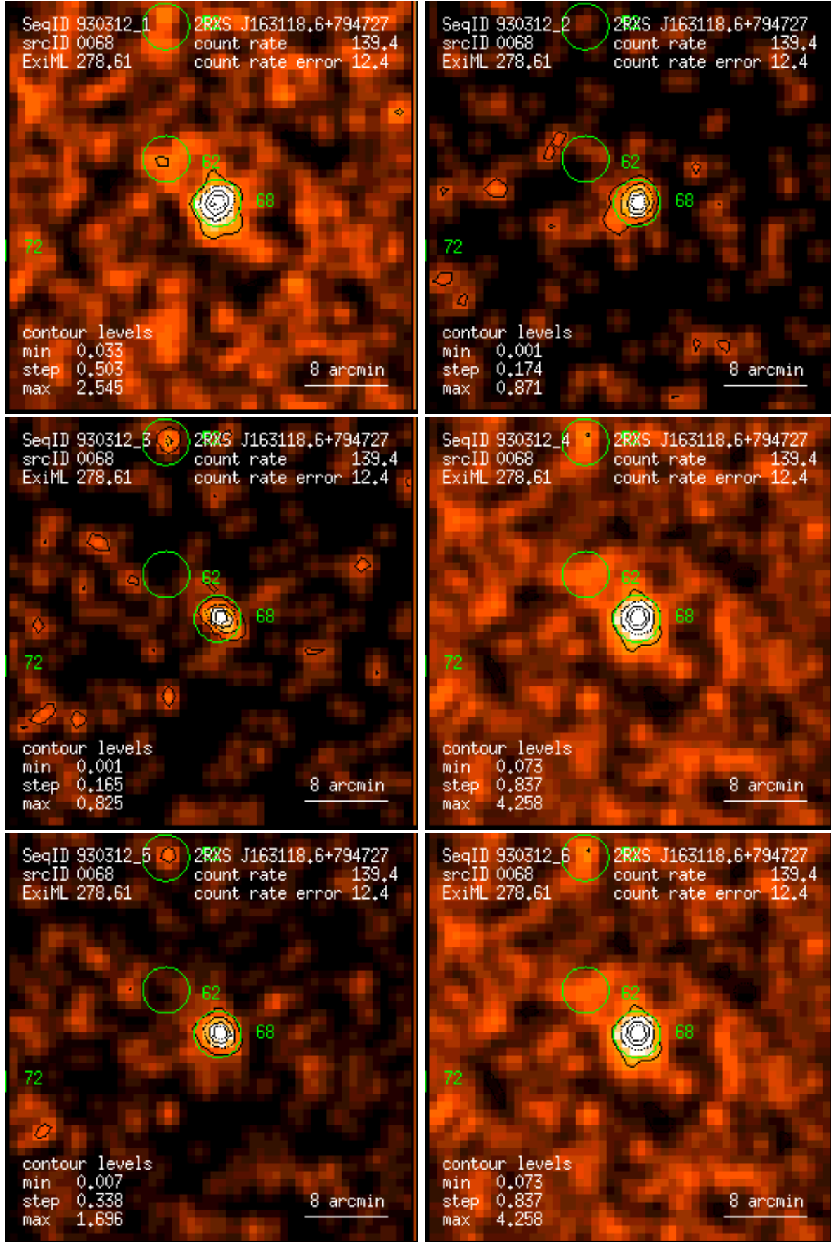
Figure 68: RASS 930312: detection 0068: band rate images, Gaussian filter: (1) PSPC channels 11 – 41, (2) 52 – 90, (3) 91 – 201, (4) 11 – 235, (5) 52 – 201, (6) 11 – 201. Broad band rates in counts/ks. Band rate contour levels in counts/ks/arcmin 2 .
