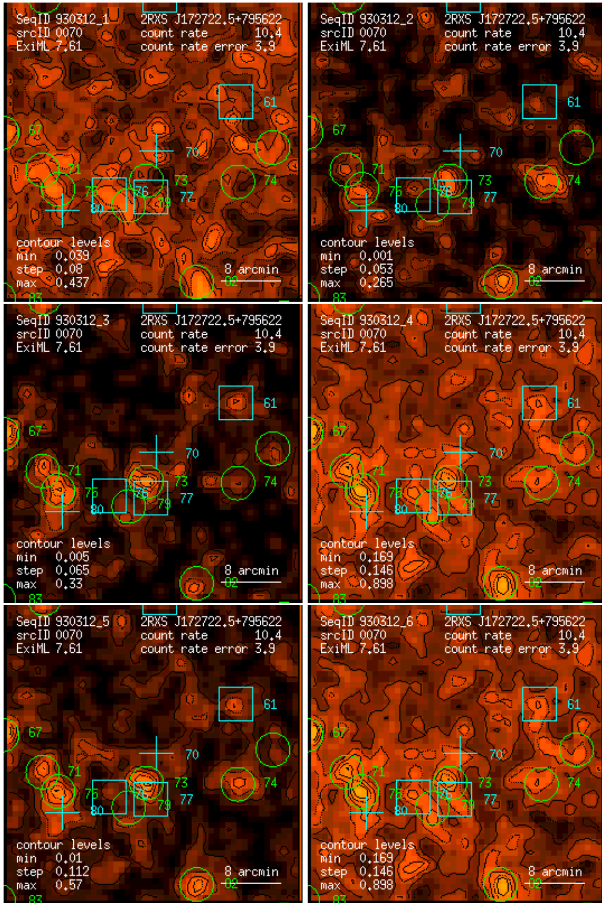
Figure 70: RASS 930312: detection 0070: band rate images, Gaussian filter: (1) PSPC channels 11 – 41, (2) 52 – 90, (3) 91 – 201, (4) 11 – 235, (5) 52 – 201, (6) 11 – 201. Broad band rates in counts/ks. Band rate contour levels in counts/ks/arcmin 2 .
