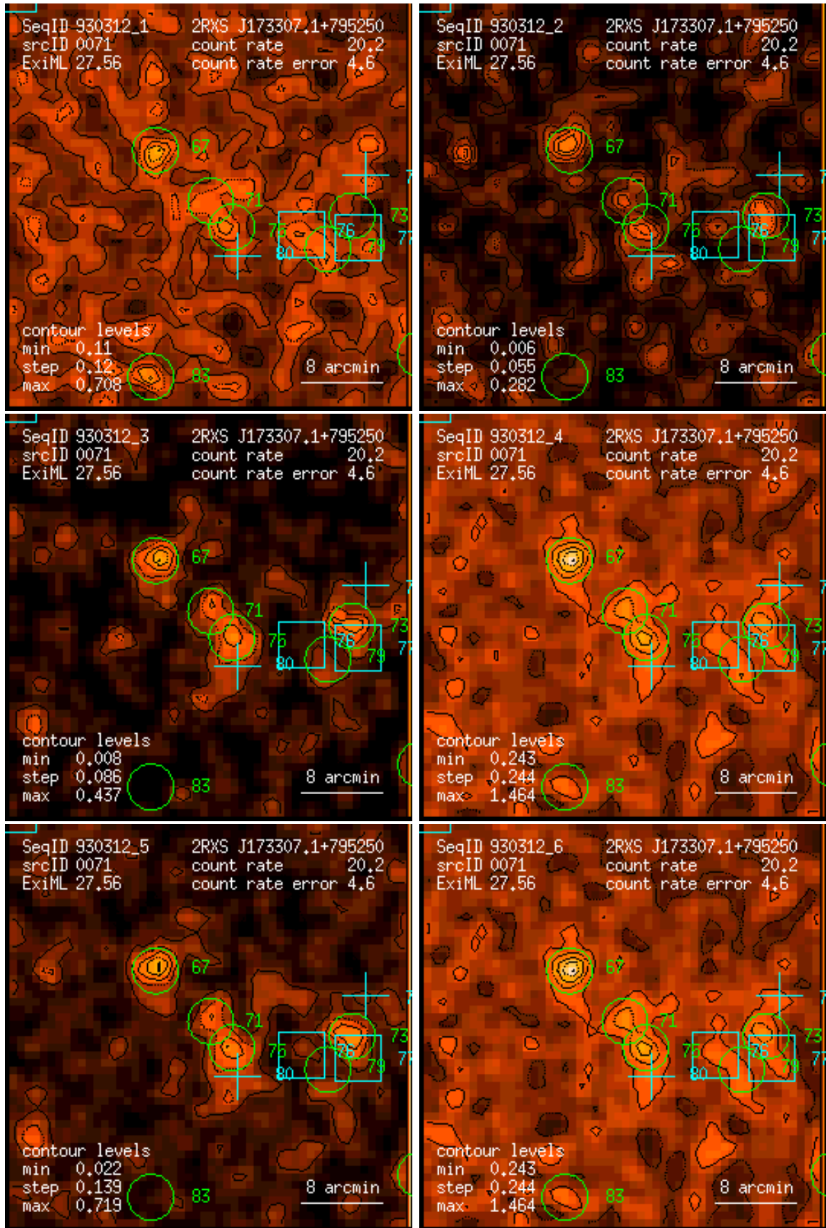
Figure 71: RASS 930312: detection 0071: band rate images, Gaussian filter: (1) PSPC channels 11 – 41, (2) 52 – 90, (3) 91 – 201, (4) 11 – 235, (5) 52 – 201, (6) 11 – 201. Broad band rates in counts/ks. Band rate contour levels in counts/ks/arcmin 2 .
