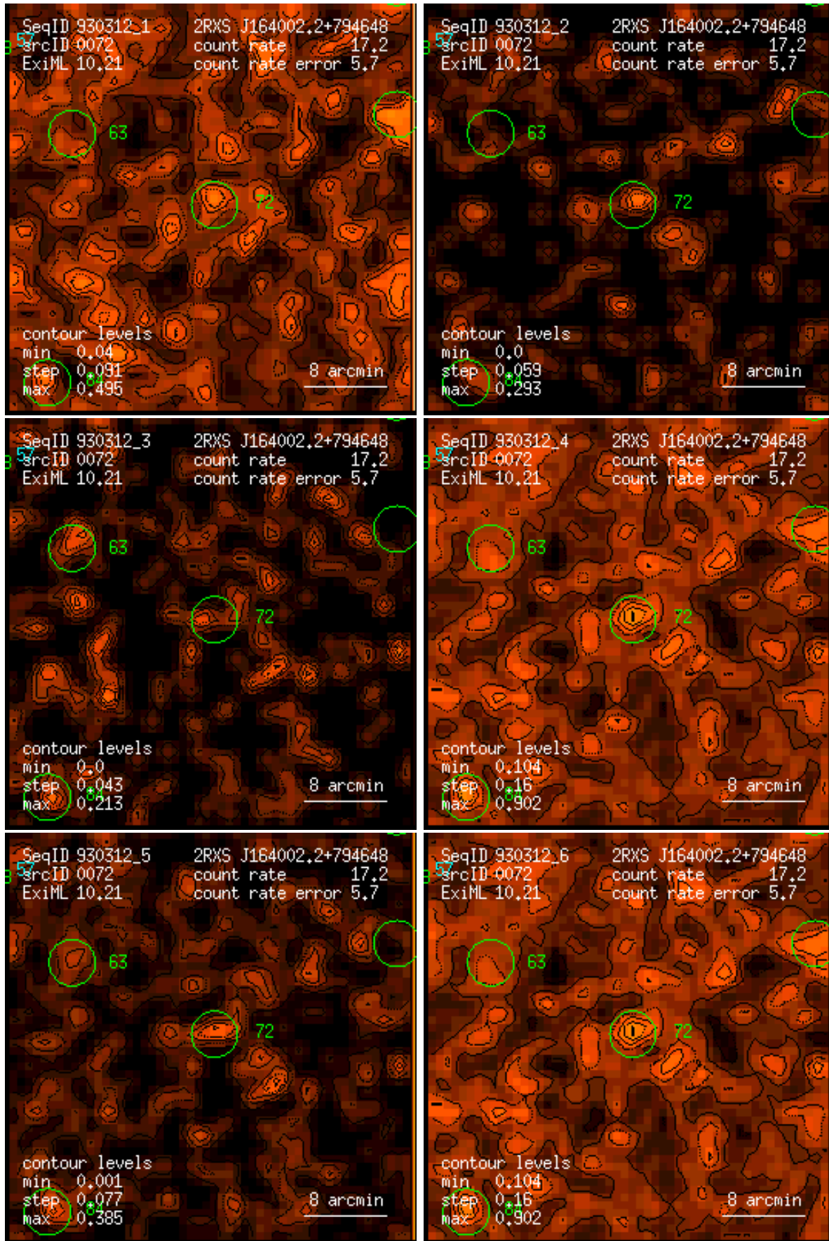
Figure 72: RASS 930312: detection 0072: band rate images, Gaussian filter: (1) PSPC channels 11 – 41, (2) 52 – 90, (3) 91 – 201, (4) 11 – 235, (5) 52 – 201, (6) 11 – 201. Broad band rates in counts/ks. Band rate contour levels in counts/ks/arcmin 2 .
