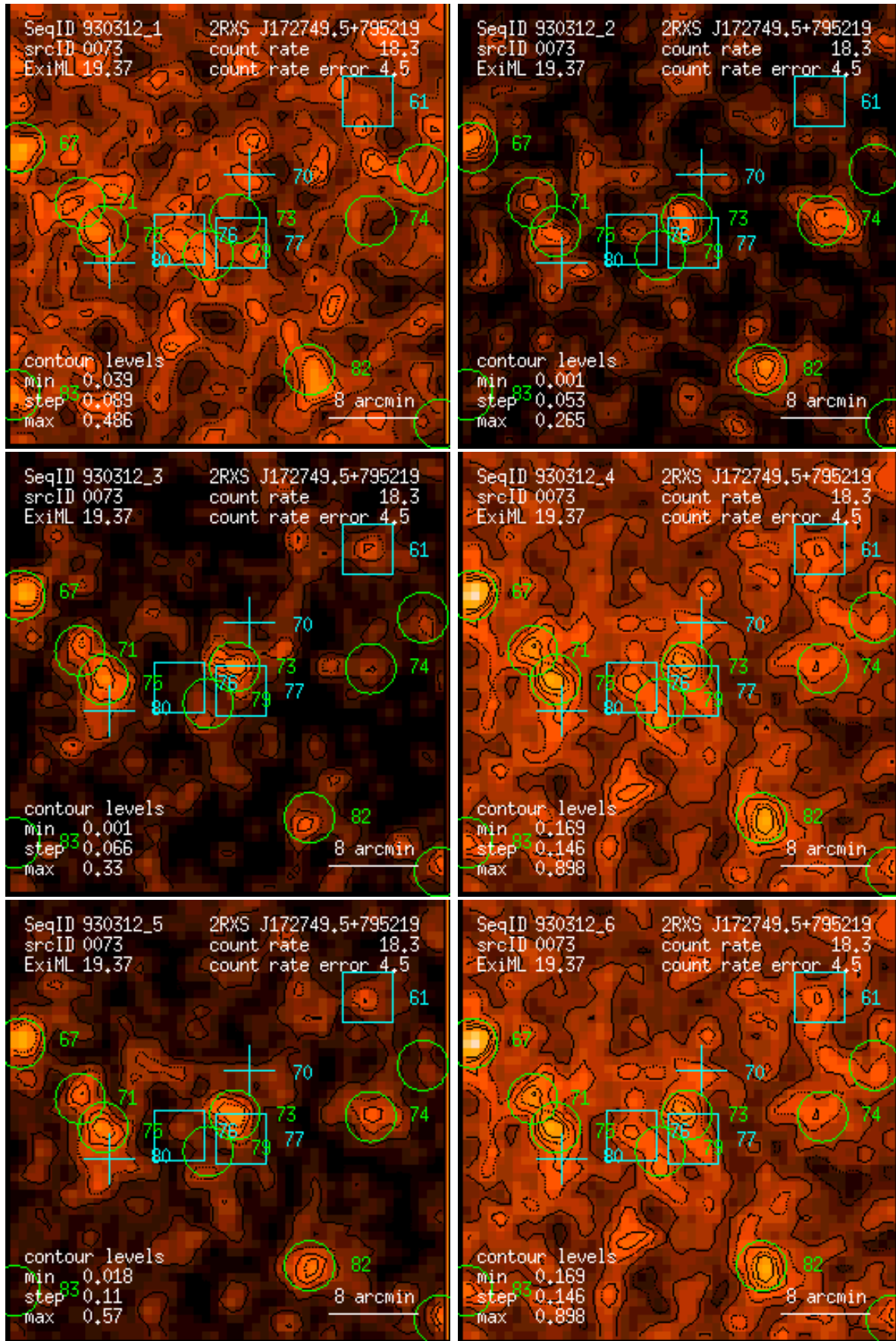
Figure 73: RASS 930312: detection 0073: band rate images, Gaussian filter: (1) PSPC channels 11 – 41, (2) 52 – 90, (3) 91 – 201, (4) 11 – 235, (5) 52 – 201, (6) 11 – 201. Broad band rates in counts/ks. Band rate contour levels in counts/ks/arcmin 2 .
