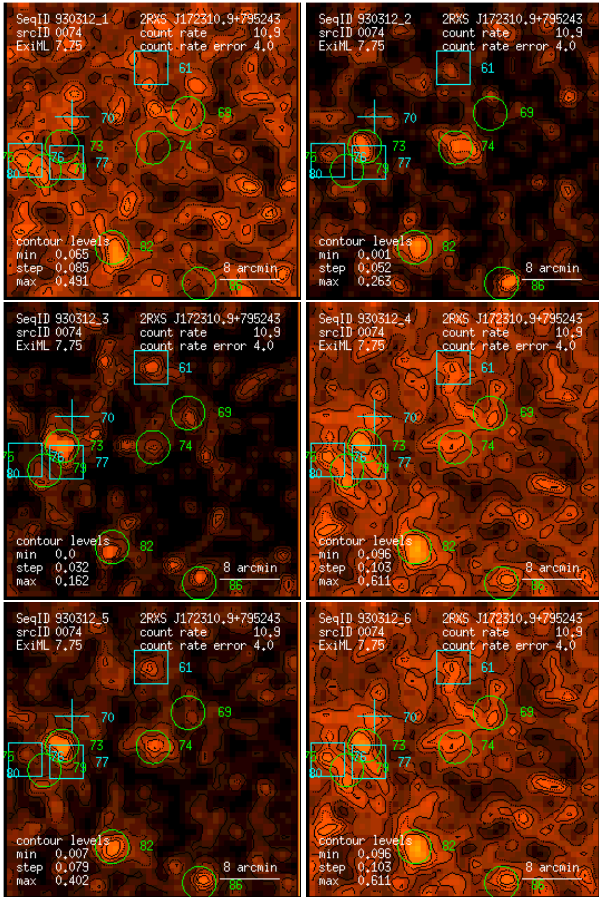
Figure 74: RASS 930312: detection 0074: band rate images, Gaussian filter: (1) PSPC channels 11 – 41, (2) 52 – 90, (3) 91 – 201, (4) 11 – 235, (5) 52 – 201, (6) 11 – 201. Broad band rates in counts/ks. Band rate contour levels in counts/ks/arcmin 2 .
