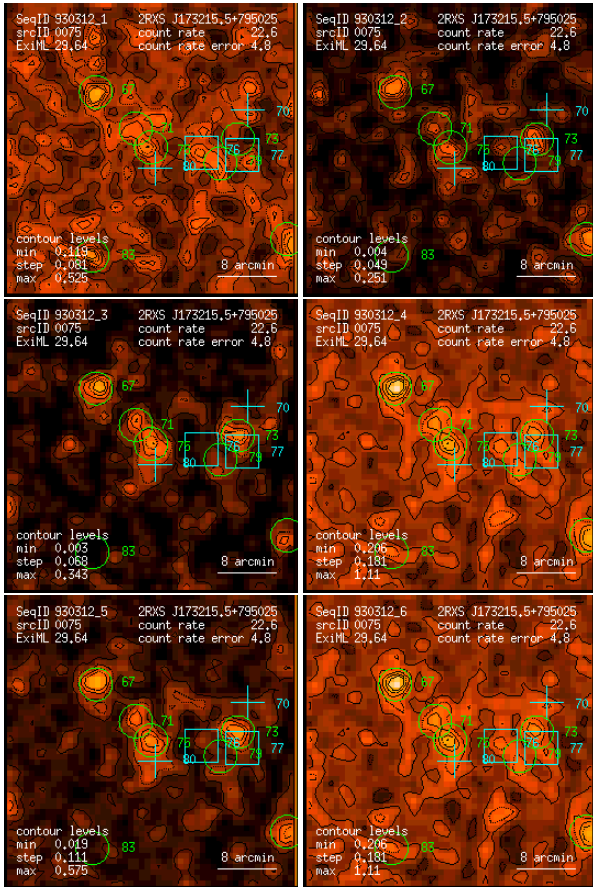
Figure 75: RASS 930312: detection 0075: band rate images, Gaussian filter: (1) PSPC channels 11 – 41, (2) 52 – 90, (3) 91 – 201, (4) 11 – 235, (5) 52 – 201, (6) 11 – 201. Broad band rates in counts/ks. Band rate contour levels in counts/ks/arcmin 2 .
