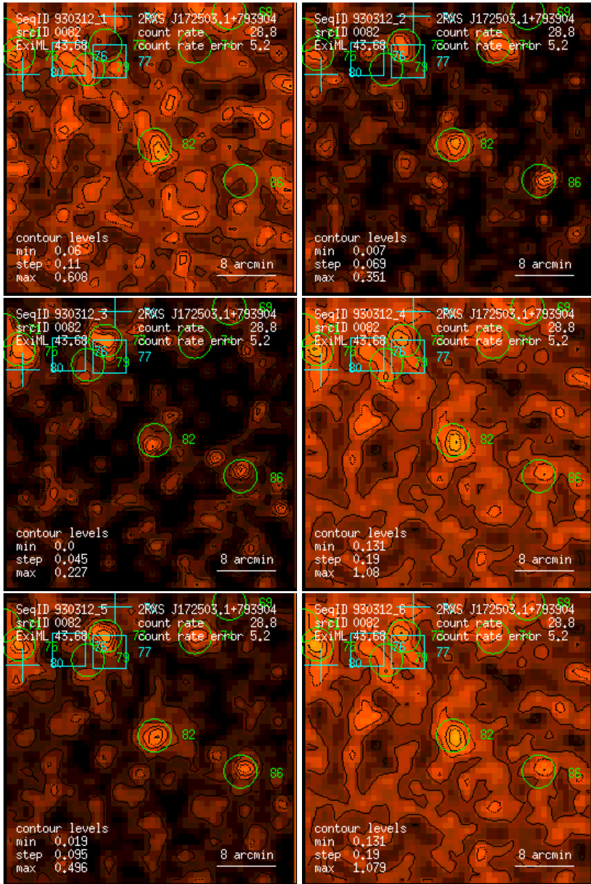
Figure 82: RASS 930312: detection 0082: band rate images, Gaussian filter: (1) PSPC channels 11 – 41, (2) 52 – 90, (3) 91 – 201, (4) 11 – 235, (5) 52 – 201, (6) 11 – 201. Broad band rates in counts/ks. Band rate contour levels in counts/ks/arcmin 2 .
