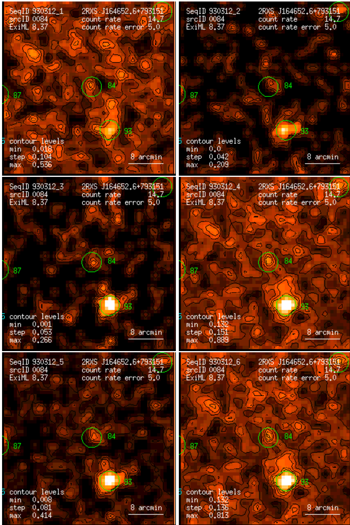
Figure 84: RASS 930312: detection 0084: band rate images, Gaussian filter: (1) PSPC channels 11 – 41, (2) 52 – 90, (3) 91 – 201, (4) 11 – 235, (5) 52 – 201, (6) 11 – 201. Broad band rates in counts/ks. Band rate contour levels in counts/ks/arcmin 2 .
