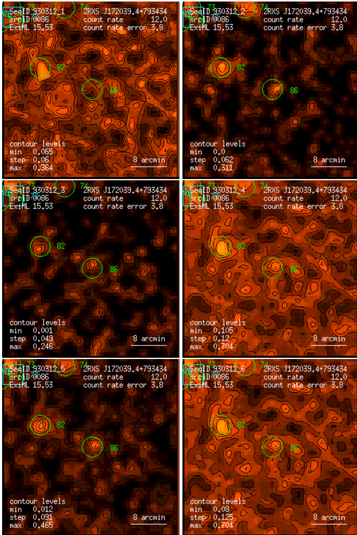
Figure 86: RASS 930312: detection 0086: band rate images, Gaussian filter: (1) PSPC channels 11 – 41, (2) 52 – 90, (3) 91 – 201, (4) 11 – 235, (5) 52 – 201, (6) 11 – 201. Broad band rates in counts/ks. Band rate contour levels in counts/ks/arcmin 2 .
