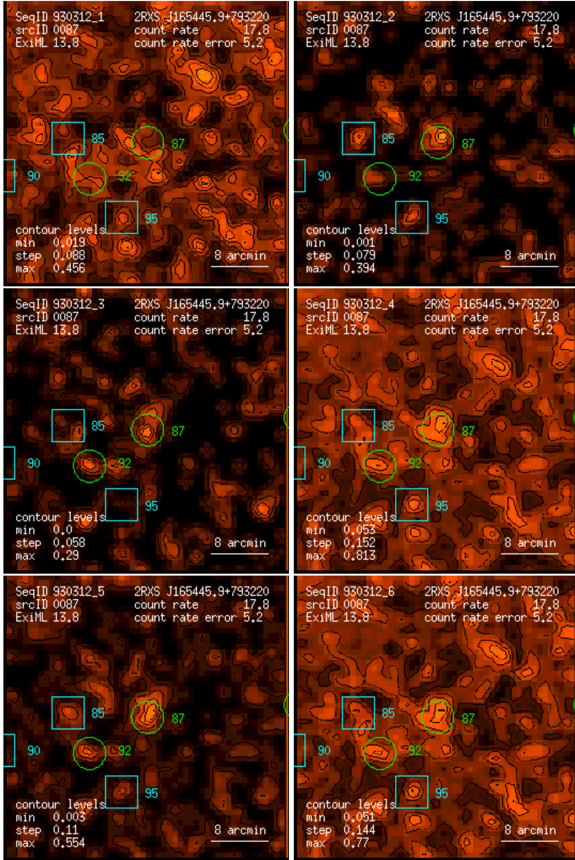
Figure 87: RASS 930312: detection 0087: band rate images, Gaussian filter: (1) PSPC channels 11 – 41, (2) 52 – 90, (3) 91 – 201, (4) 11 – 235, (5) 52 – 201, (6) 11 – 201. Broad band rates in counts/ks. Band rate contour levels in counts/ks/arcmin 2 .
