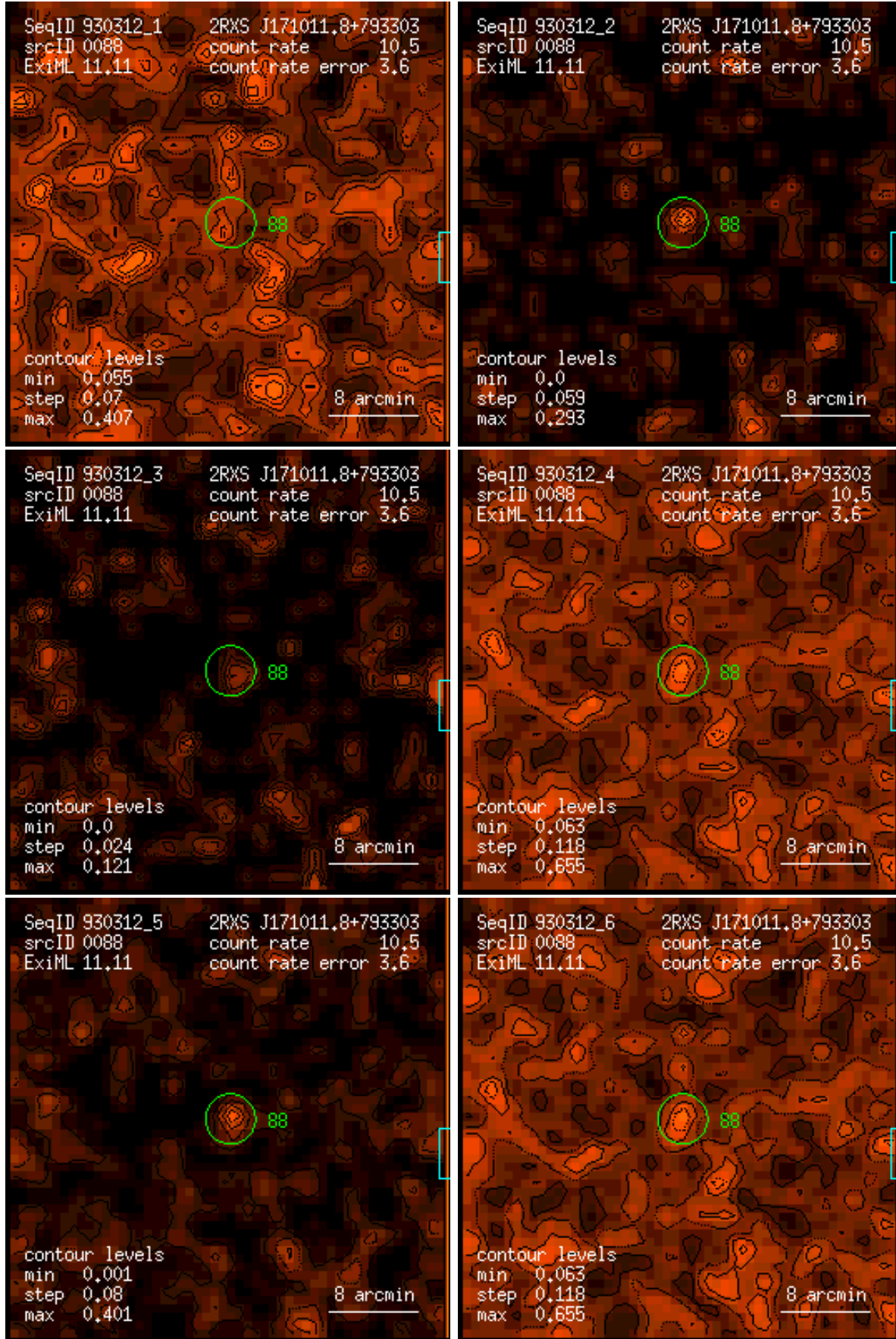
Figure 88: RASS 930312: detection 0088: band rate images, Gaussian filter: (1) PSPC channels 11 – 41, (2) 52 – 90, (3) 91 – 201, (4) 11 – 235, (5) 52 – 201, (6) 11 – 201. Broad band rates in counts/ks. Band rate contour levels in counts/ks/arcmin 2 .
