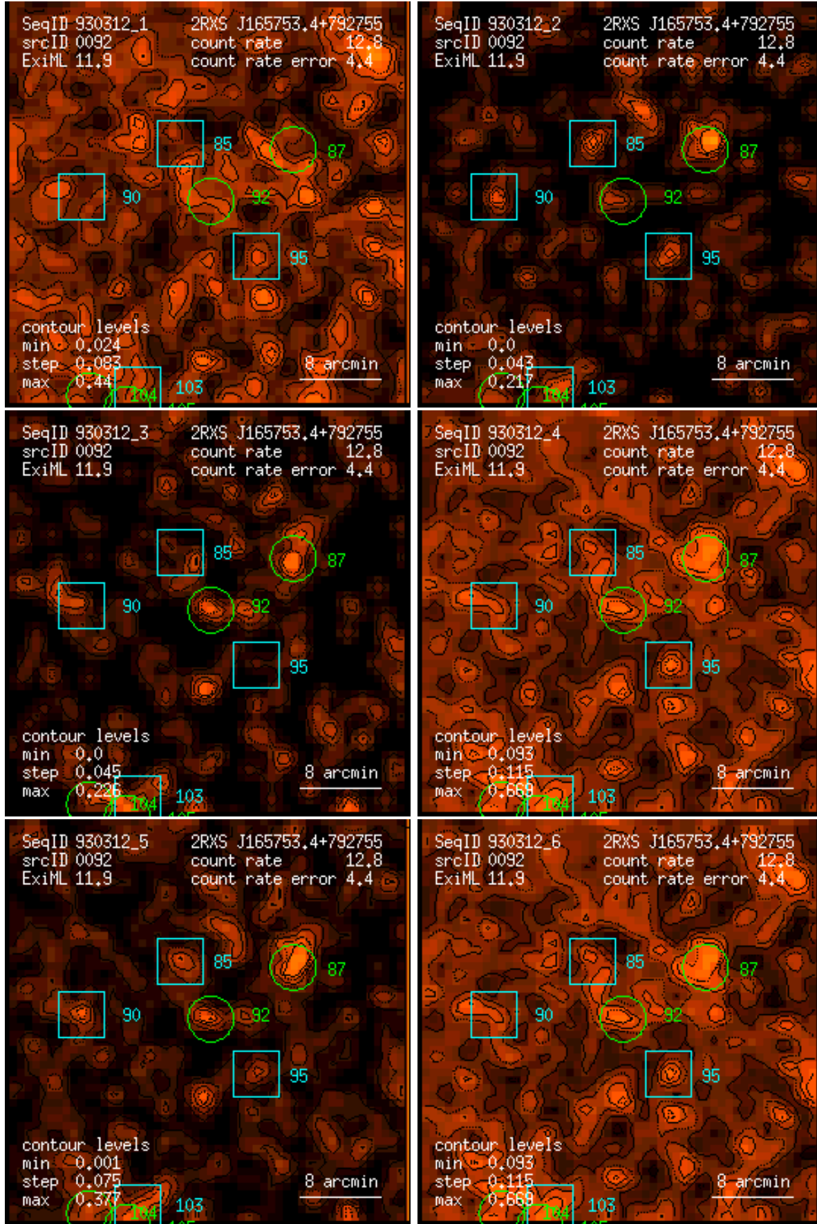
Figure 92: RASS 930312: detection 0092: band rate images, Gaussian filter: (1) PSPC channels 11 – 41, (2) 52 – 90, (3) 91 – 201, (4) 11 – 235, (5) 52 – 201, (6) 11 – 201. Broad band rates in counts/ks. Band rate contour levels in counts/ks/arcmin 2 .
