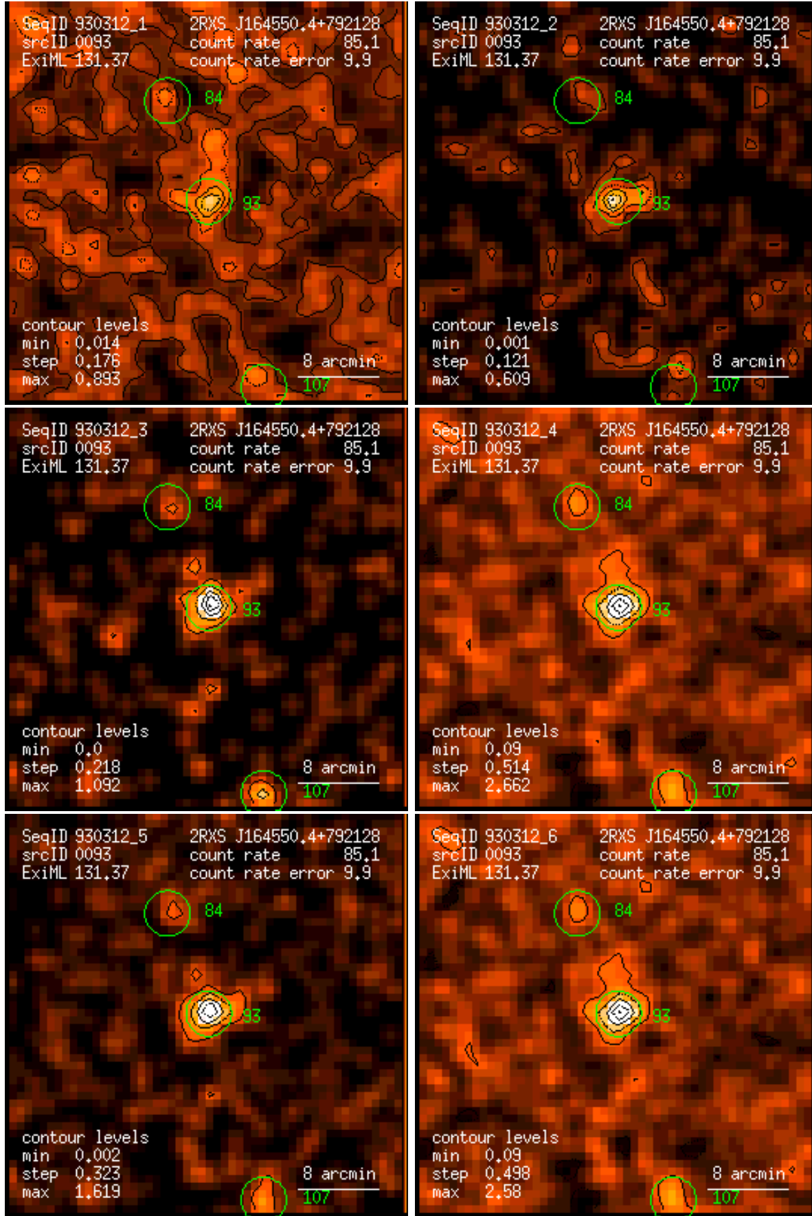
Figure 93: RASS 930312: detection 0093: band rate images, Gaussian filter: (1) PSPC channels 11 – 41, (2) 52 – 90, (3) 91 – 201, (4) 11 – 235, (5) 52 – 201, (6) 11 – 201. Broad band rates in counts/ks. Band rate contour levels in counts/ks/arcmin 2 .
