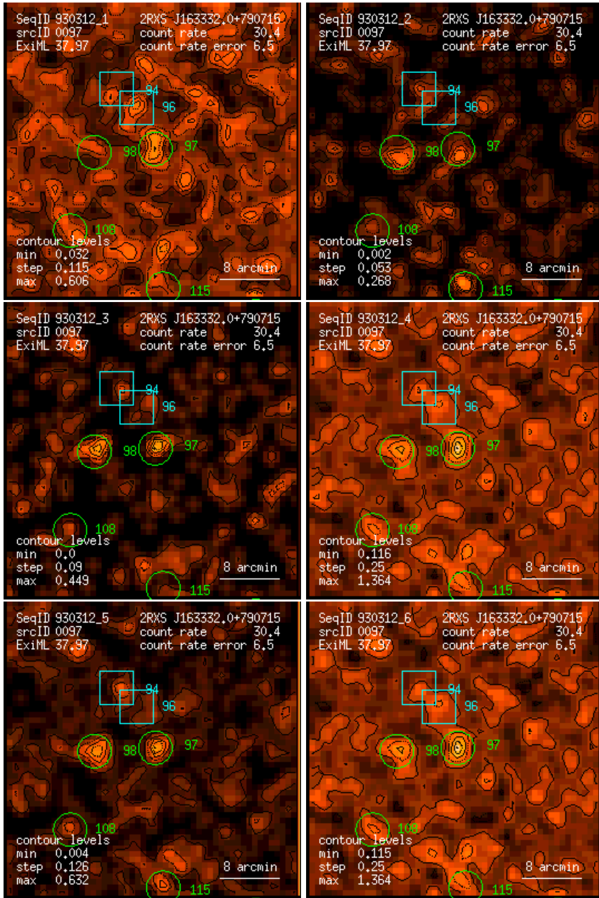
Figure 97: RASS 930312: detection 0097: band rate images, Gaussian filter: (1) PSPC channels 11 – 41, (2) 52 – 90, (3) 91 – 201, (4) 11 – 235, (5) 52 – 201, (6) 11 – 201. Broad band rates in counts/ks. Band rate contour levels in counts/ks/arcmin 2 .
