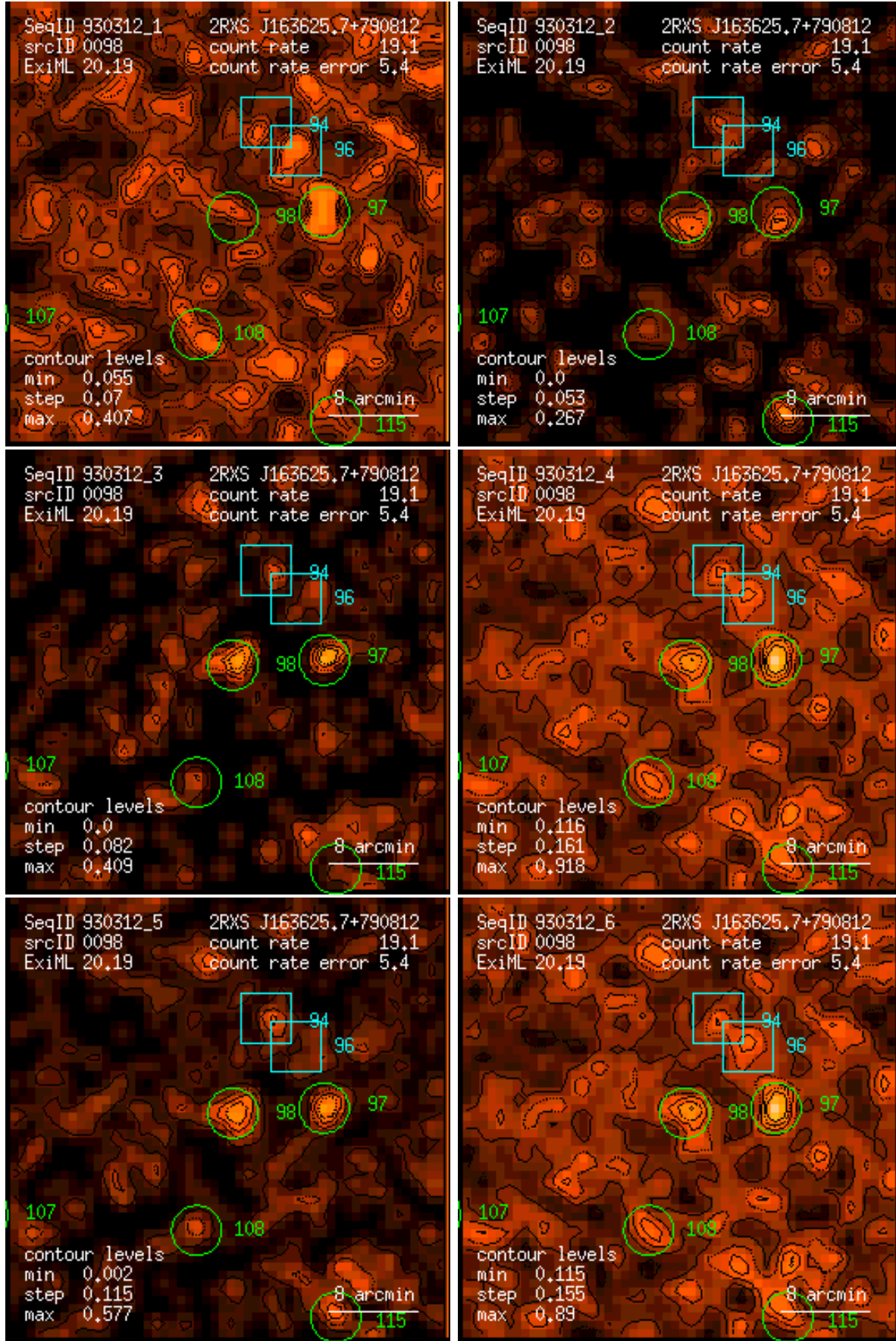
Figure 98: RASS 930312: detection 0098: band rate images, Gaussian filter: (1) PSPC channels 11 – 41, (2) 52 – 90, (3) 91 – 201, (4) 11 – 235, (5) 52 – 201, (6) 11 – 201. Broad band rates in counts/ks. Band rate contour levels in counts/ks/arcmin 2 .
