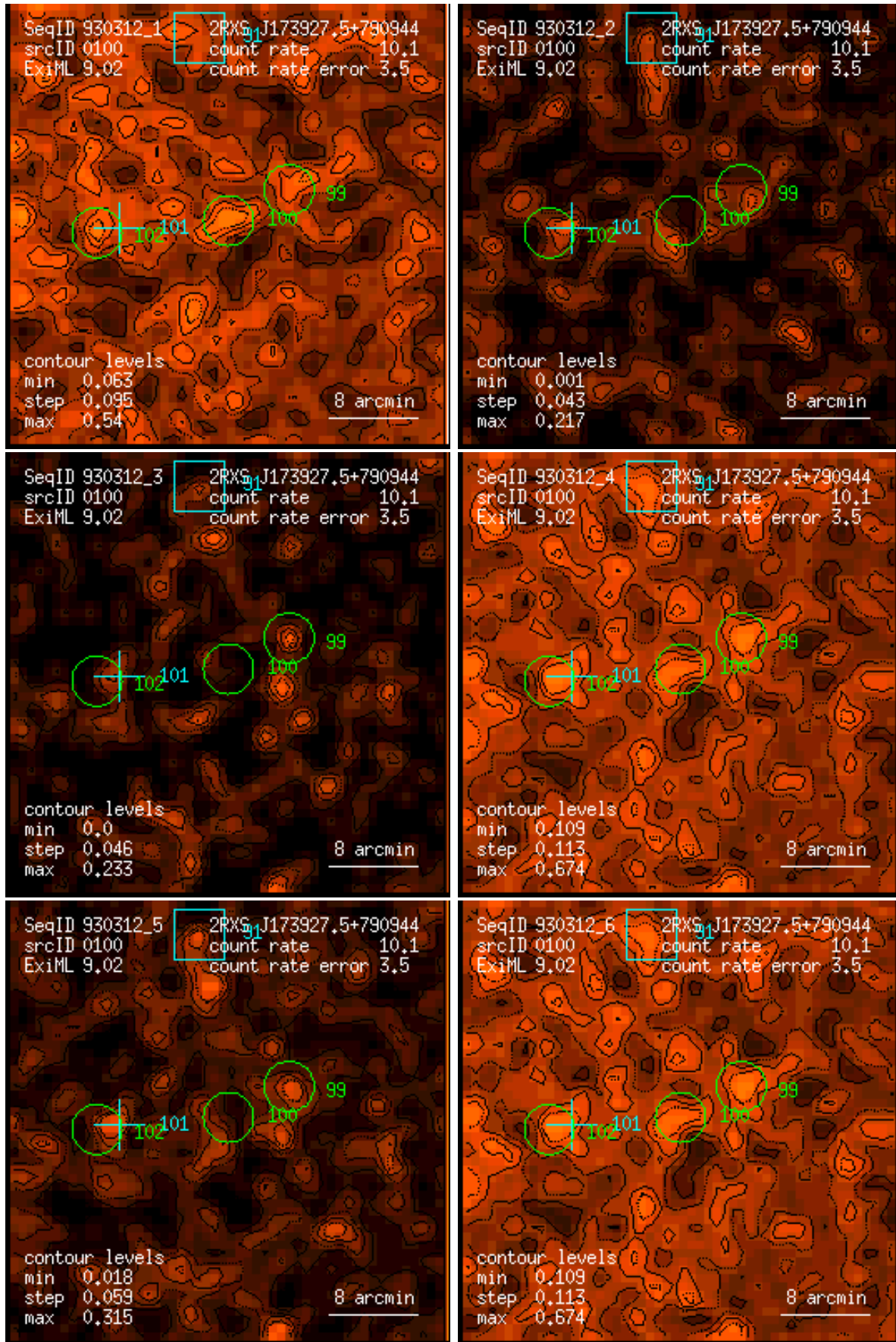
Figure 100: RASS 930312: detection 0100: band rate images, Gaussian filter: (1) PSPC channels 11 – 41, (2) 52 – 90, (3) 91 – 201, (4) 11 – 235, (5) 52 – 201, (6) 11 – 201. Broad band rates in counts/ks. Band rate contour levels in counts/ks/arcmin 2 .
