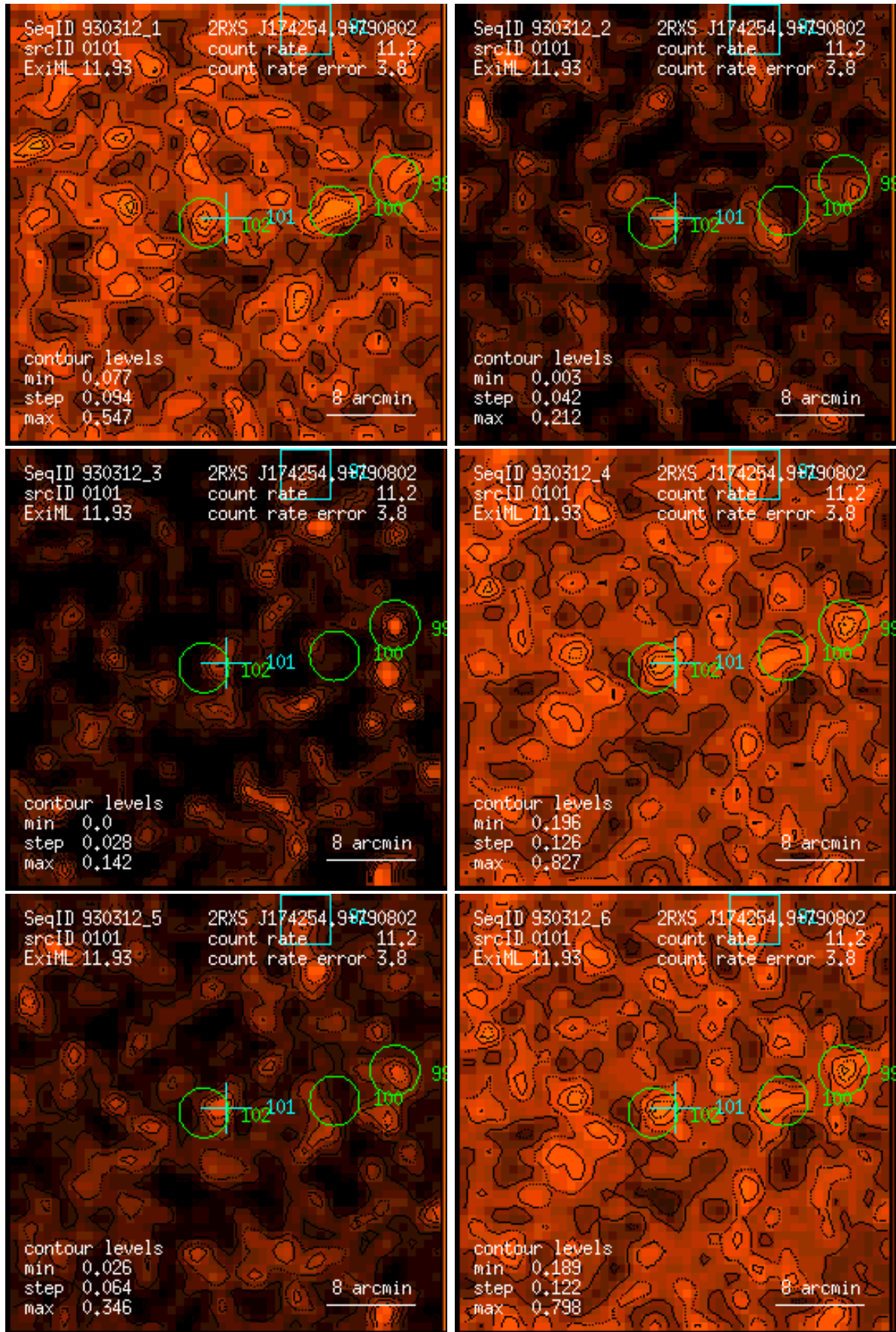
Figure 101: RASS 930312: detection 0101: band rate images, Gaussian filter: (1) PSPC channels 11 – 41, (2) 52 – 90, (3) 91 – 201, (4) 11 – 235, (5) 52 – 201, (6) 11 – 201. Broad band rates in counts/ks. Band rate contour levels in counts/ks/arcmin 2 .
