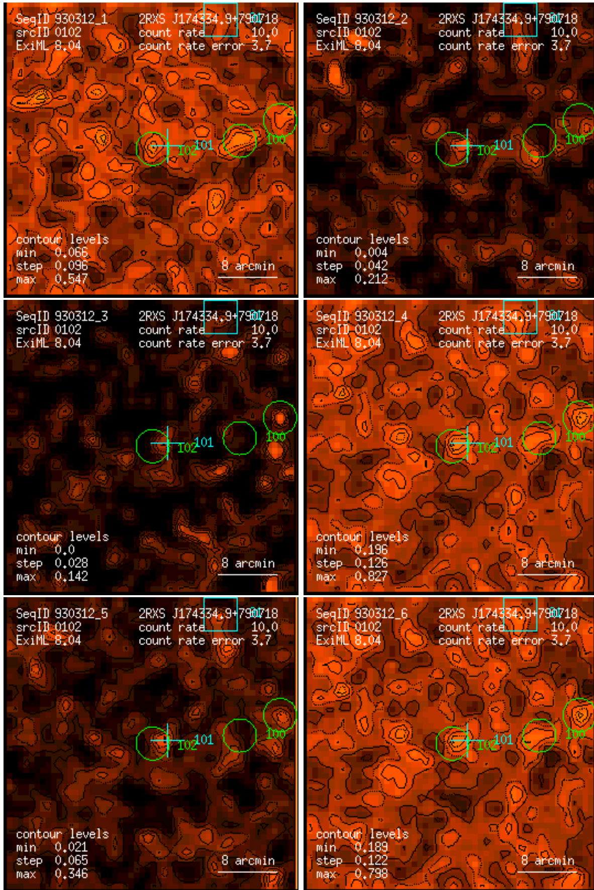
Figure 102: RASS 930312: detection 0102: band rate images, Gaussian filter: (1) PSPC channels 11 – 41, (2) 52 – 90, (3) 91 – 201, (4) 11 – 235, (5) 52 – 201, (6) 11 – 201. Broad band rates in counts/ks. Band rate contour levels in counts/ks/arcmin 2 .
