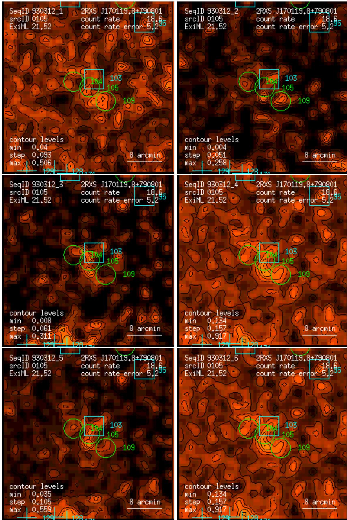
Figure 105: RASS 930312: detection 0105: band rate images, Gaussian filter: (1) PSPC channels 11 – 41, (2) 52 – 90, (3) 91 – 201, (4) 11 – 235, (5) 52 – 201, (6) 11 – 201. Broad band rates in counts/ks. Band rate contour levels in counts/ks/arcmin 2 .
