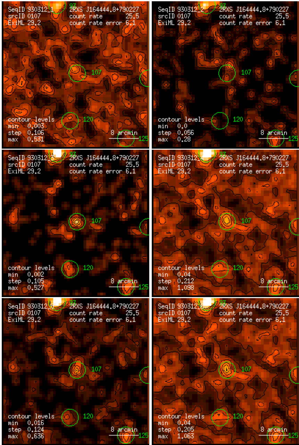
Figure 107: RASS 930312: detection 0107: band rate images, Gaussian filter: (1) PSPC channels 11 – 41, (2) 52 – 90, (3) 91 – 201, (4) 11 – 235, (5) 52 – 201, (6) 11 – 201. Broad band rates in counts/ks. Band rate contour levels in counts/ks/arcmin 2 .
