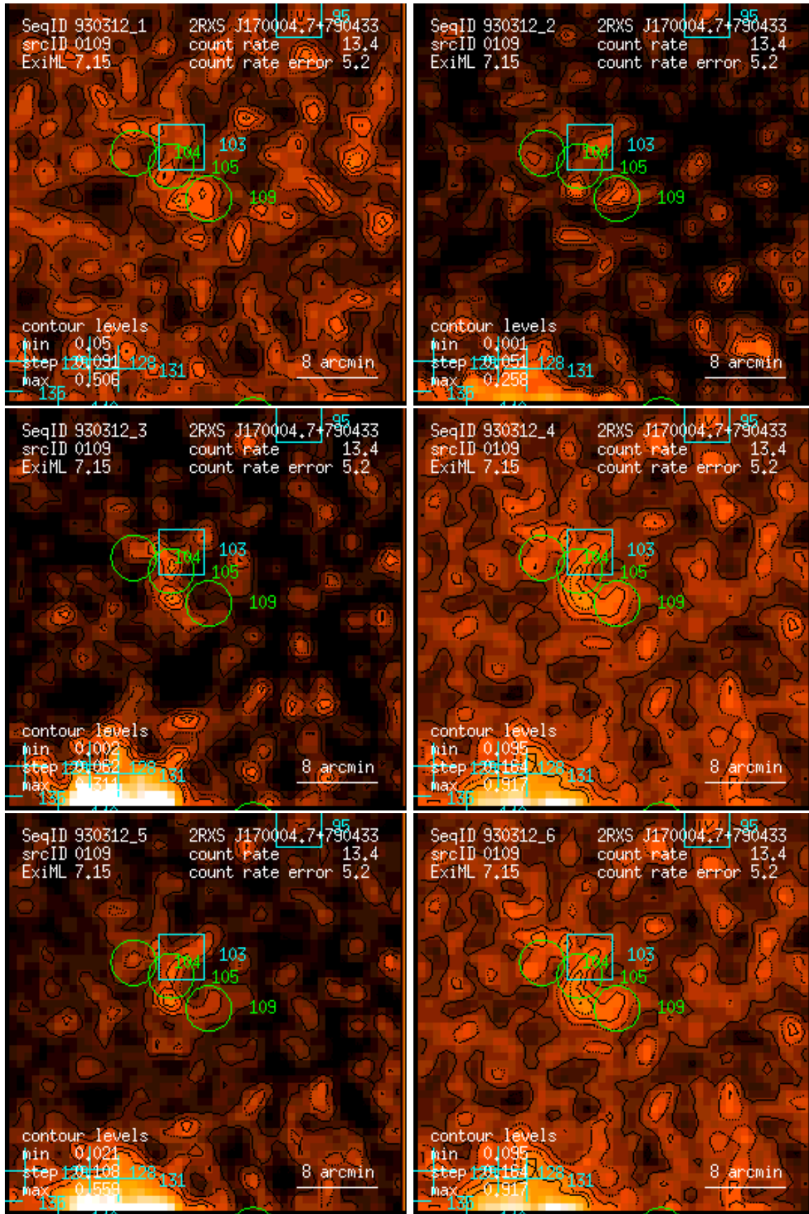
Figure 109: RASS 930312: detection 0109: band rate images, Gaussian filter: (1) PSPC channels 11 – 41, (2) 52 – 90, (3) 91 – 201, (4) 11 – 235, (5) 52 – 201, (6) 11 – 201. Broad band rates in counts/ks. Band rate contour levels in counts/ks/arcmin 2 .
