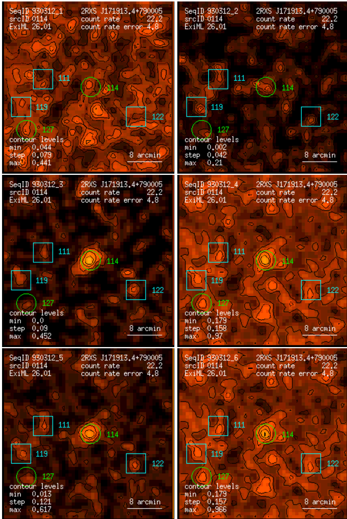
Figure 114: RASS 930312: detection 0114: band rate images, Gaussian filter: (1) PSPC channels 11 – 41, (2) 52 – 90, (3) 91 – 201, (4) 11 – 235, (5) 52 – 201, (6) 11 – 201. Broad band rates in counts/ks. Band rate contour levels in counts/ks/arcmin 2 .
