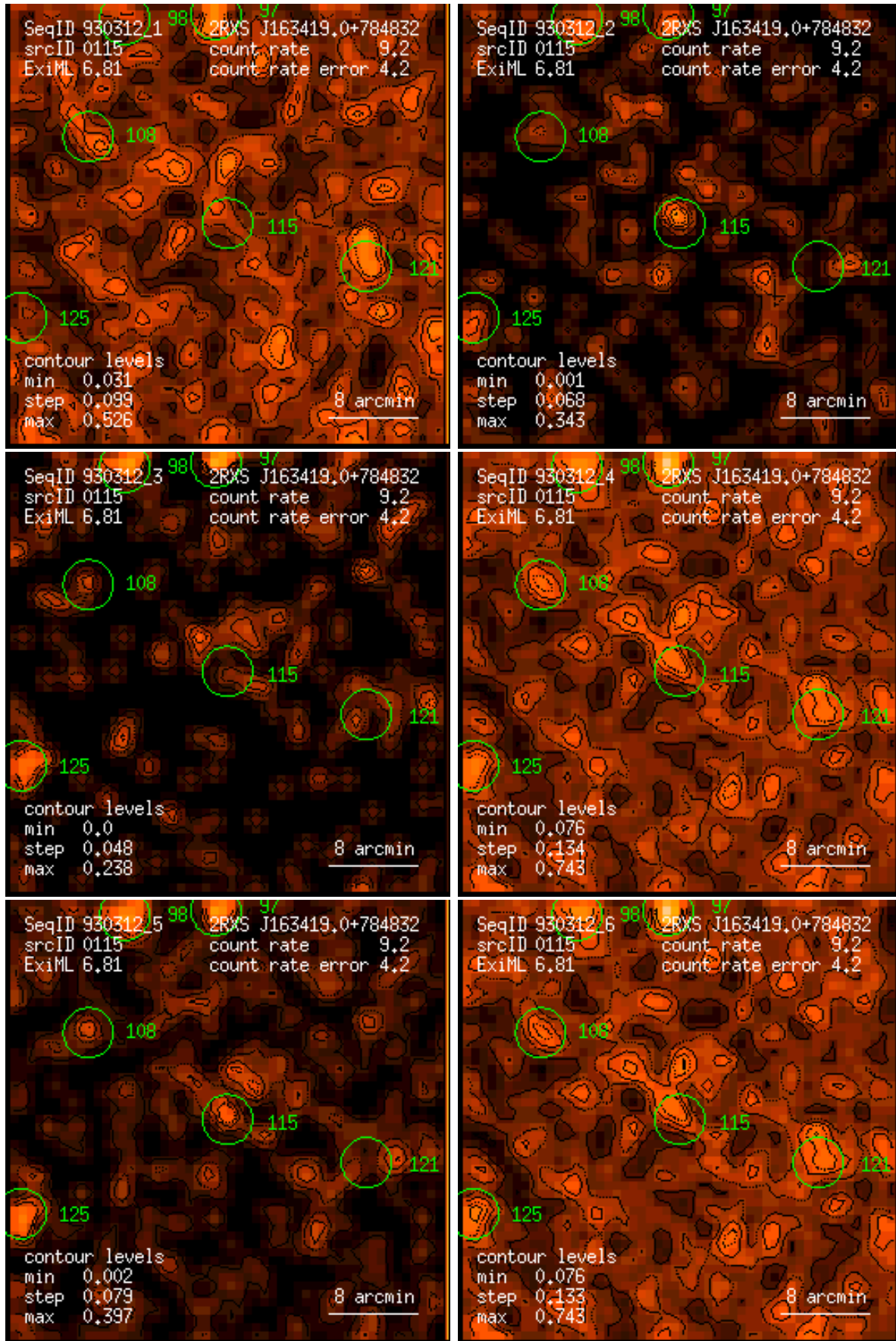
Figure 115: RASS 930312: detection 0115: band rate images, Gaussian filter: (1) PSPC channels 11 – 41, (2) 52 – 90, (3) 91 – 201, (4) 11 – 235, (5) 52 – 201, (6) 11 – 201. Broad band rates in counts/ks. Band rate contour levels in counts/ks/arcmin 2 .
