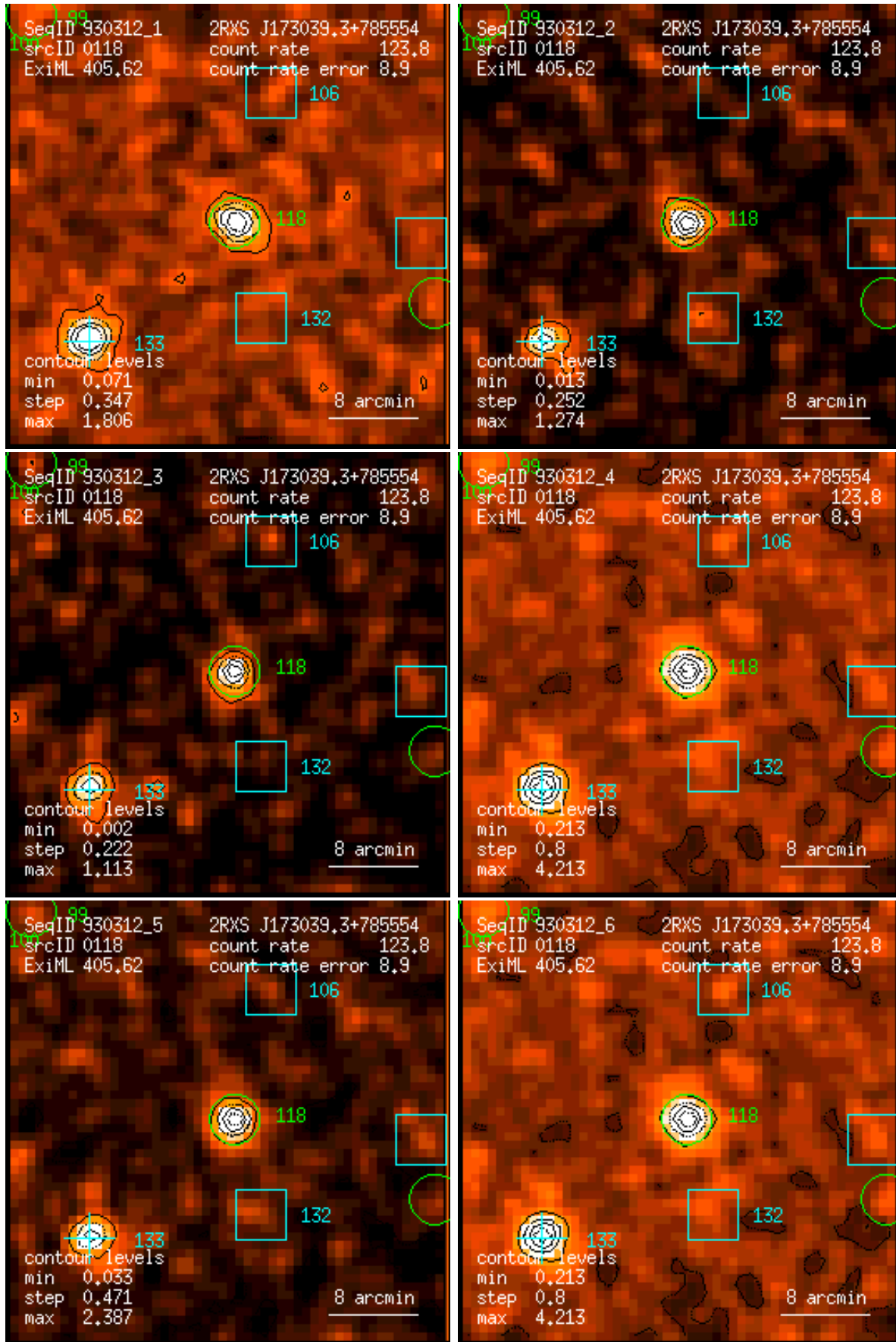
Figure 118: RASS 930312: detection 0118: band rate images, Gaussian filter: (1) PSPC channels 11 – 41, (2) 52 – 90, (3) 91 – 201, (4) 11 – 235, (5) 52 – 201, (6) 11 – 201. Broad band rates in counts/ks. Band rate contour levels in counts/ks/arcmin 2 .
