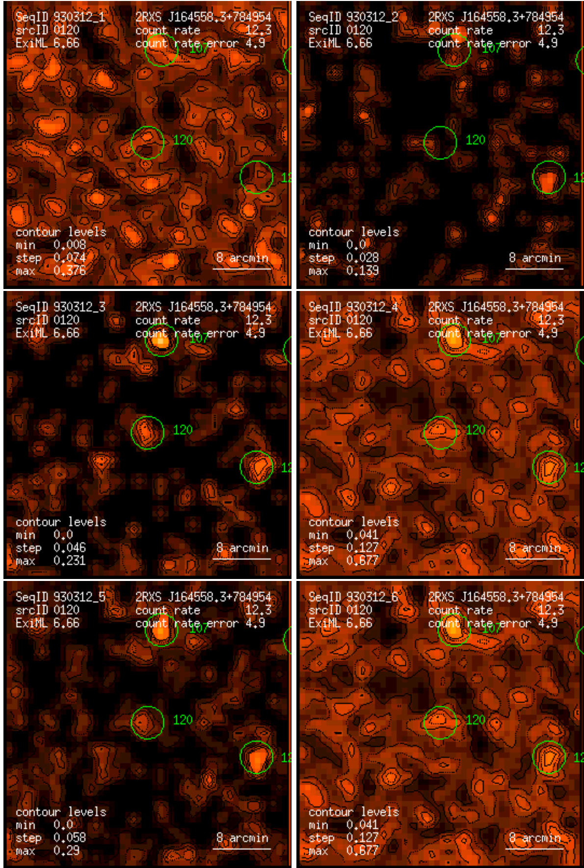
Figure 120: RASS 930312: detection 0120: band rate images, Gaussian filter: (1) PSPC channels 11 – 41, (2) 52 – 90, (3) 91 – 201, (4) 11 – 235, (5) 52 – 201, (6) 11 – 201. Broad band rates in counts/ks. Band rate contour levels in counts/ks/arcmin 2 .
