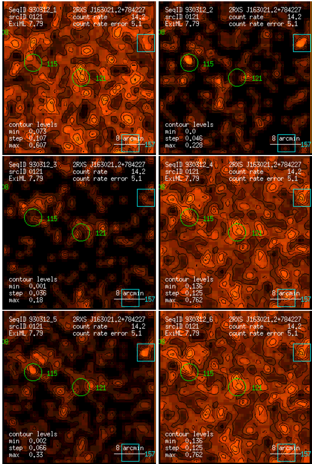
Figure 121: RASS 930312: detection 0121: band rate images, Gaussian filter: (1) PSPC channels 11 – 41, (2) 52 – 90, (3) 91 – 201, (4) 11 – 235, (5) 52 – 201, (6) 11 – 201. Broad band rates in counts/ks. Band rate contour levels in counts/ks/arcmin 2 .
