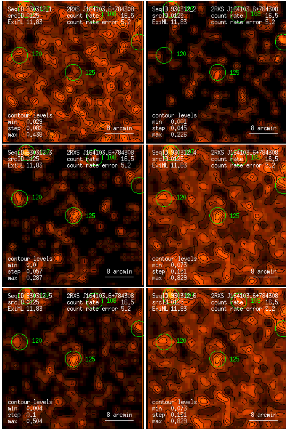
Figure 125: RASS 930312: detection 0125: band rate images, Gaussian filter: (1) PSPC channels 11 – 41, (2) 52 – 90, (3) 91 – 201, (4) 11 – 235, (5) 52 – 201, (6) 11 – 201. Broad band rates in counts/ks. Band rate contour levels in counts/ks/arcmin 2 .
