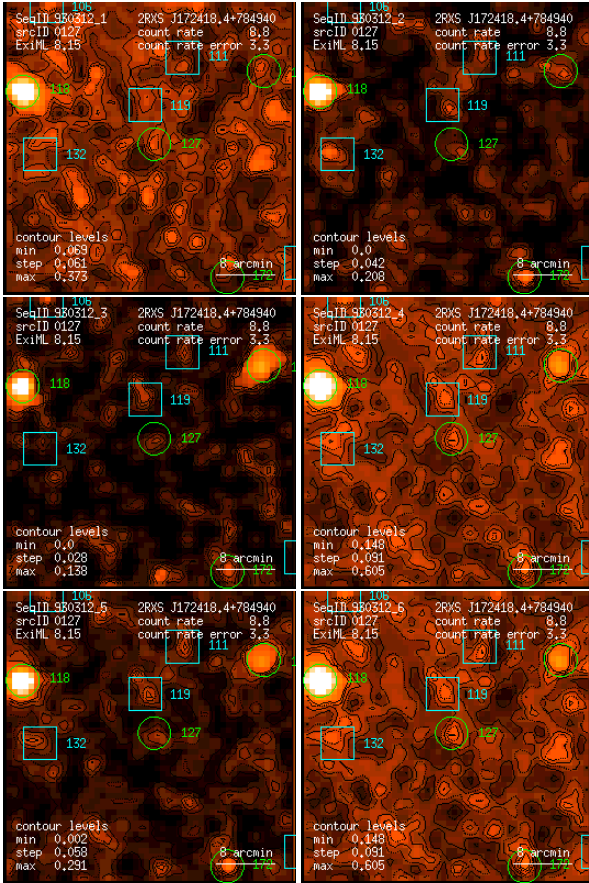
Figure 127: RASS 930312: detection 0127: band rate images, Gaussian filter: (1) PSPC channels 11 – 41, (2) 52 – 90, (3) 91 – 201, (4) 11 – 235, (5) 52 – 201, (6) 11 – 201. Broad band rates in counts/ks. Band rate contour levels in counts/ks/arcmin 2 .
