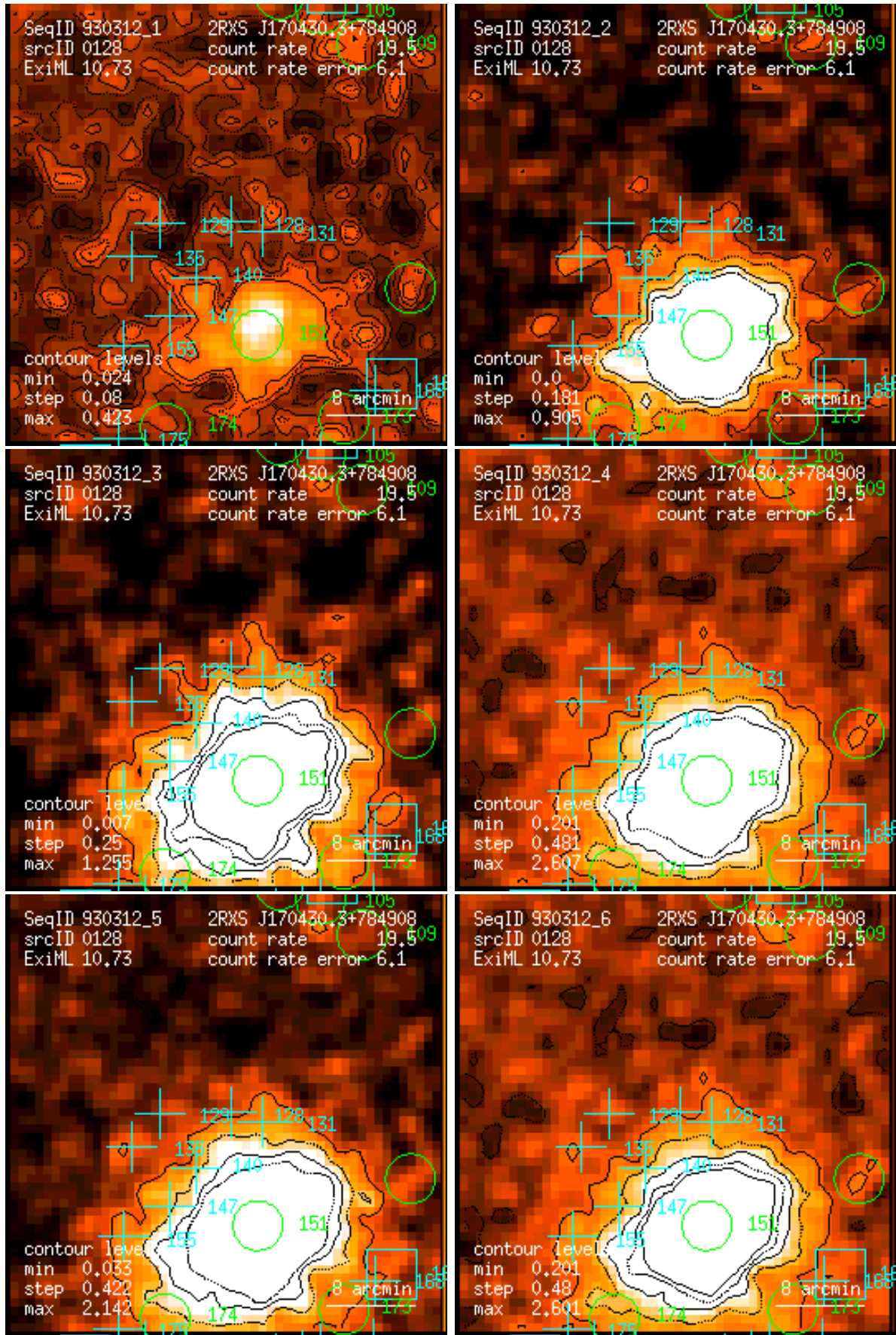
Figure 128: RASS 930312: detection 0128: band rate images, Gaussian filter: (1) PSPC channels 11 – 41, (2) 52 – 90, (3) 91 – 201, (4) 11 – 235, (5) 52 – 201, (6) 11 – 201. Broad band rates in counts/ks. Band rate contour levels in counts/ks/arcmin 2 .
