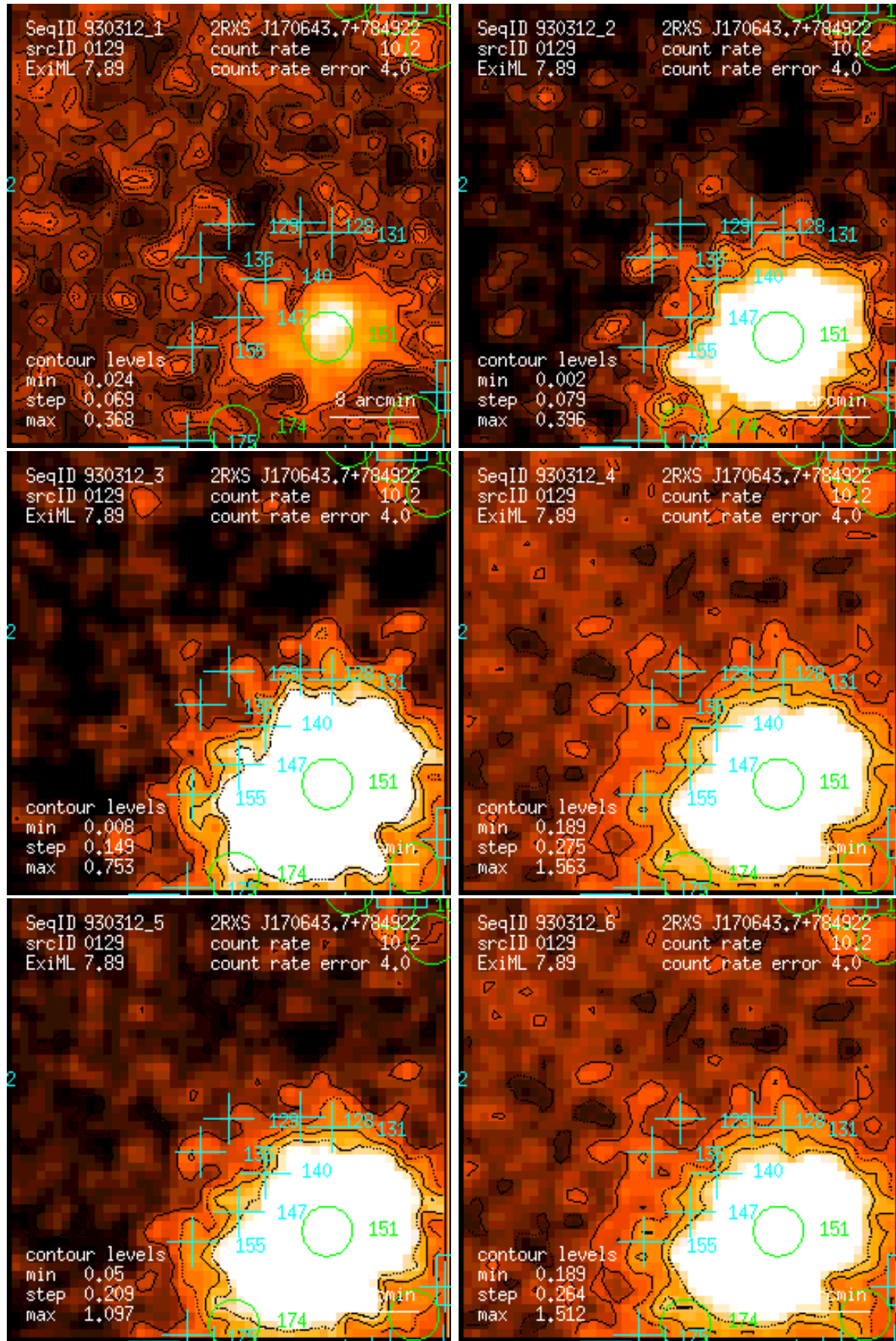
Figure 129: RASS 930312: detection 0129: band rate images, Gaussian filter: (1) PSPC channels 11 – 41, (2) 52 – 90, (3) 91 – 201, (4) 11 – 235, (5) 52 – 201, (6) 11 – 201. Broad band rates in counts/ks. Band rate contour levels in counts/ks/arcmin 2 .
