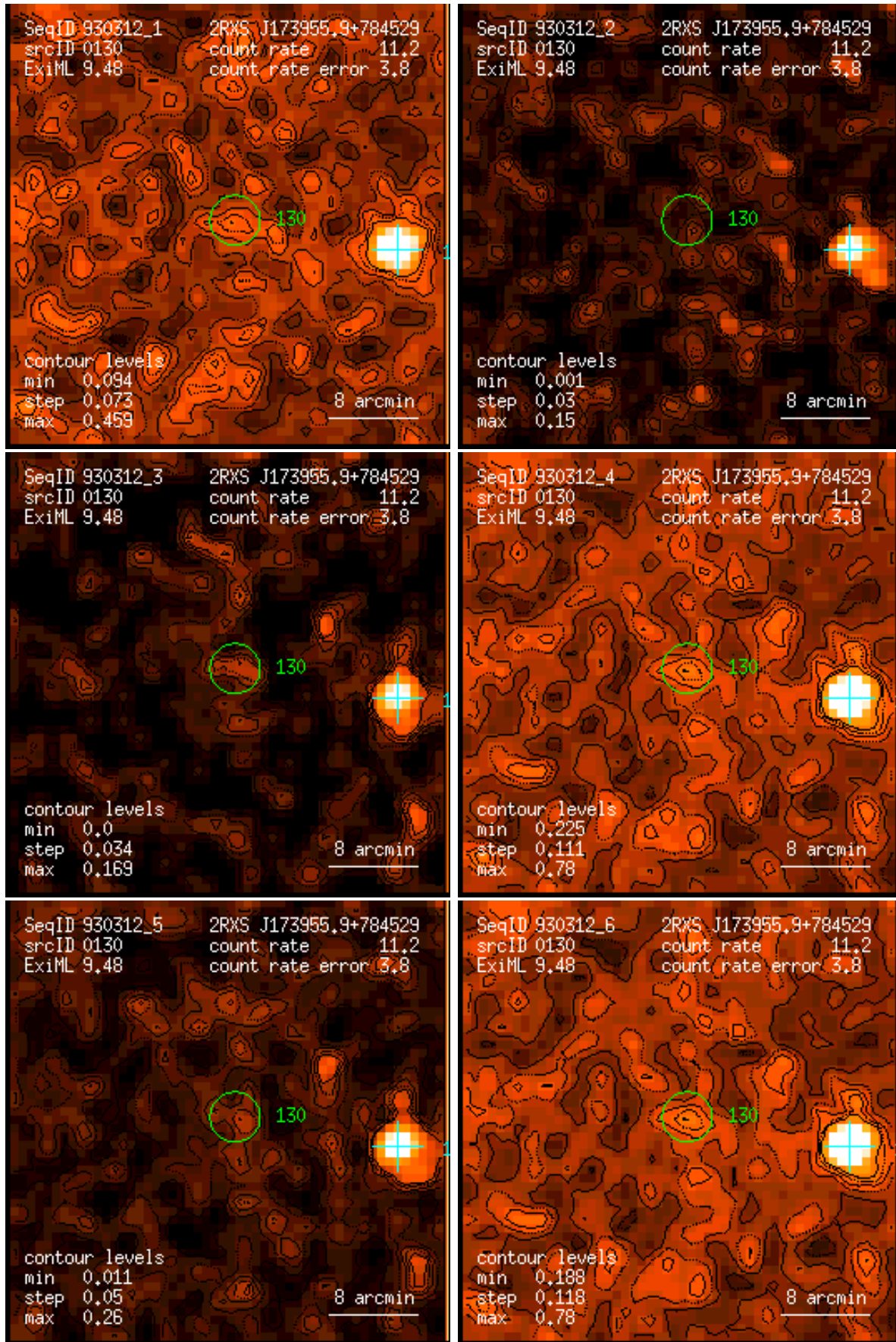
Figure 130: RASS 930312: detection 0130: band rate images, Gaussian filter: (1) PSPC channels 11 – 41, (2) 52 – 90, (3) 91 – 201, (4) 11 – 235, (5) 52 – 201, (6) 11 – 201. Broad band rates in counts/ks. Band rate contour levels in counts/ks/arcmin 2 .
