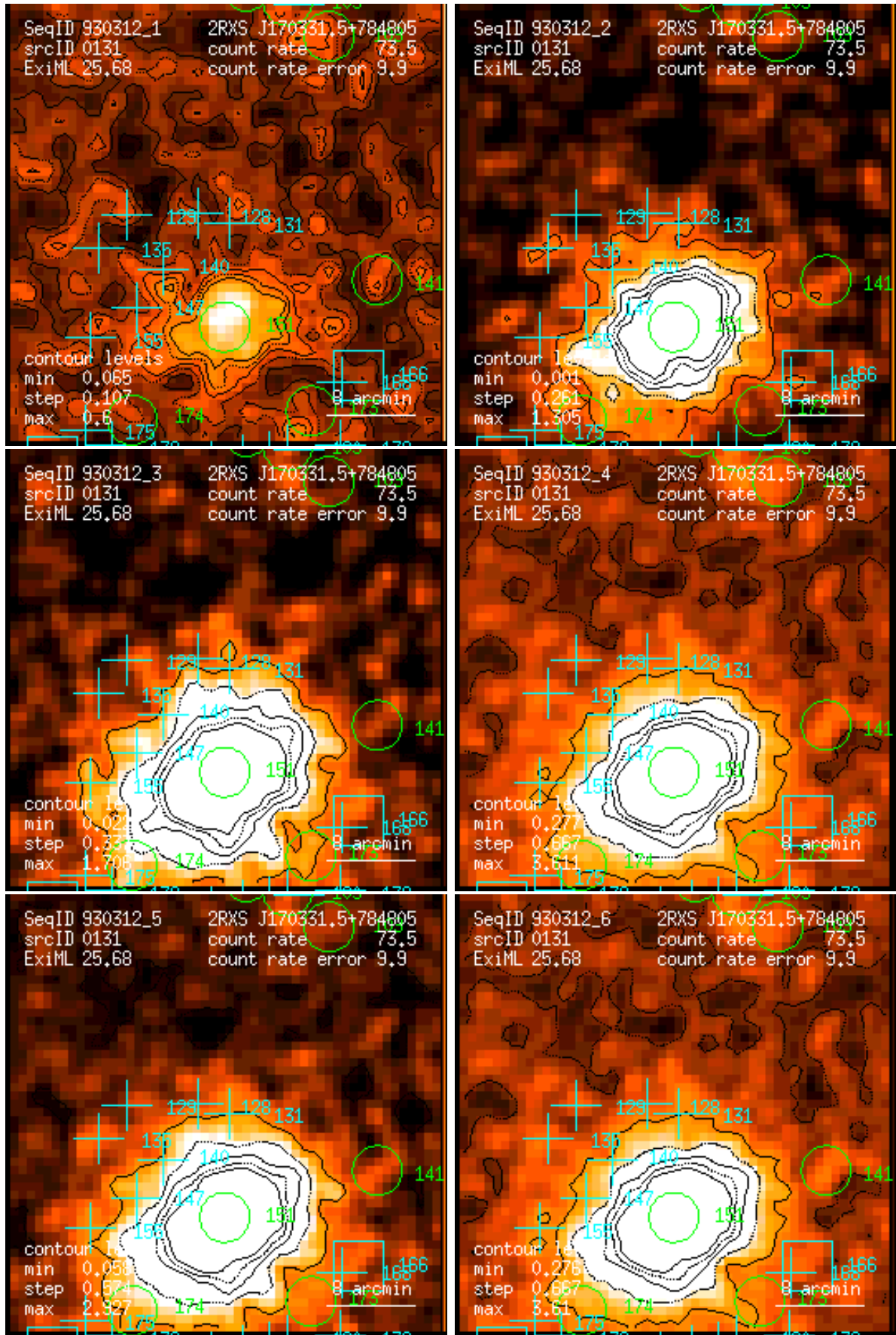
Figure 131: RASS 930312: detection 0131: band rate images, Gaussian filter: (1) PSPC channels 11 – 41, (2) 52 – 90, (3) 91 – 201, (4) 11 – 235, (5) 52 – 201, (6) 11 – 201. Broad band rates in counts/ks. Band rate contour levels in counts/ks/arcmin 2 .
