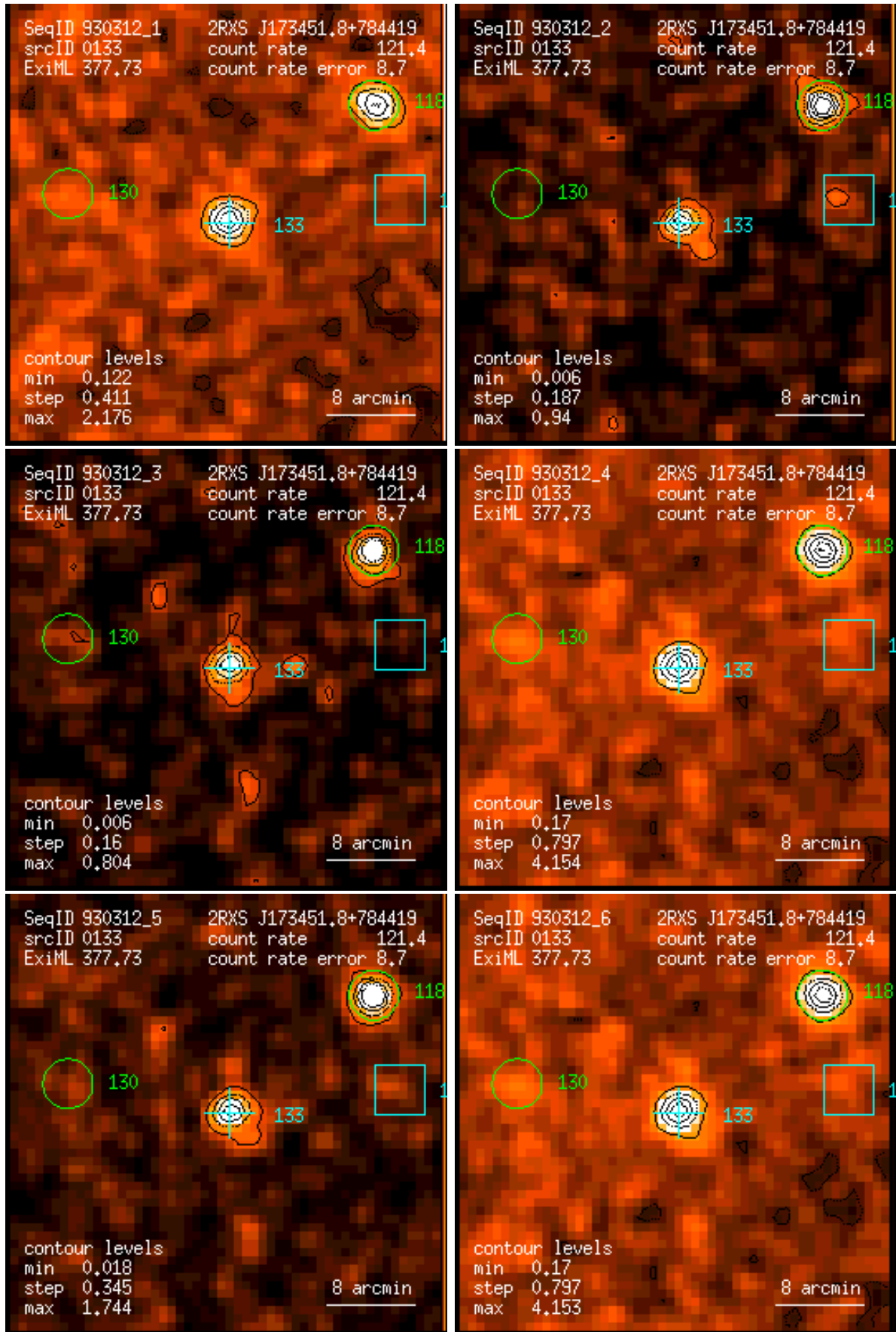
Figure 133: RASS 930312: detection 0133: band rate images, Gaussian filter: (1) PSPC channels 11 – 41, (2) 52 – 90, (3) 91 – 201, (4) 11 – 235, (5) 52 – 201, (6) 11 – 201. Broad band rates in counts/ks. Band rate contour levels in counts/ks/arcmin 2 .
