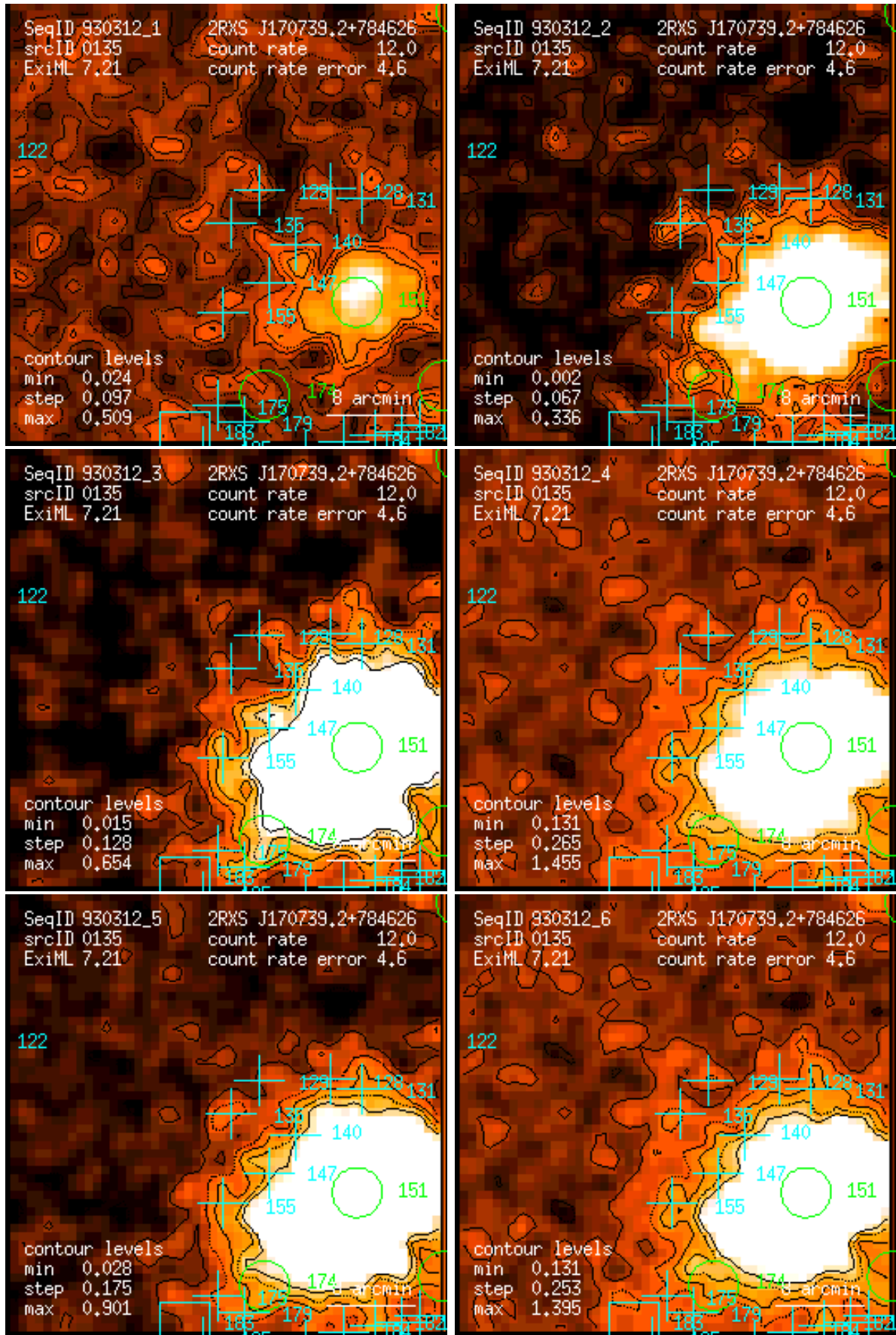
Figure 135: RASS 930312: detection 0135: band rate images, Gaussian filter: (1) PSPC channels 11 – 41, (2) 52 – 90, (3) 91 – 201, (4) 11 – 235, (5) 52 – 201, (6) 11 – 201. Broad band rates in counts/ks. Band rate contour levels in counts/ks/arcmin 2 .
