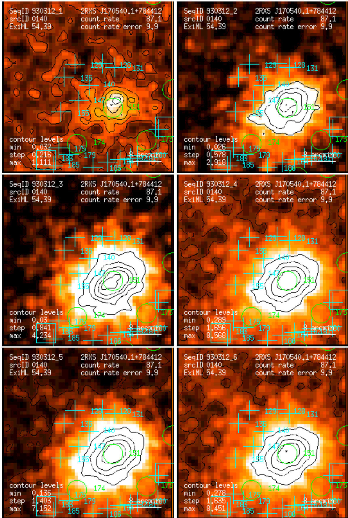
Figure 140: RASS 930312: detection 0140: band rate images, Gaussian filter: (1) PSPC channels 11 – 41, (2) 52 – 90, (3) 91 – 201, (4) 11 – 235, (5) 52 – 201, (6) 11 – 201. Broad band rates in counts/ks. Band rate contour levels in counts/ks/arcmin 2 .
