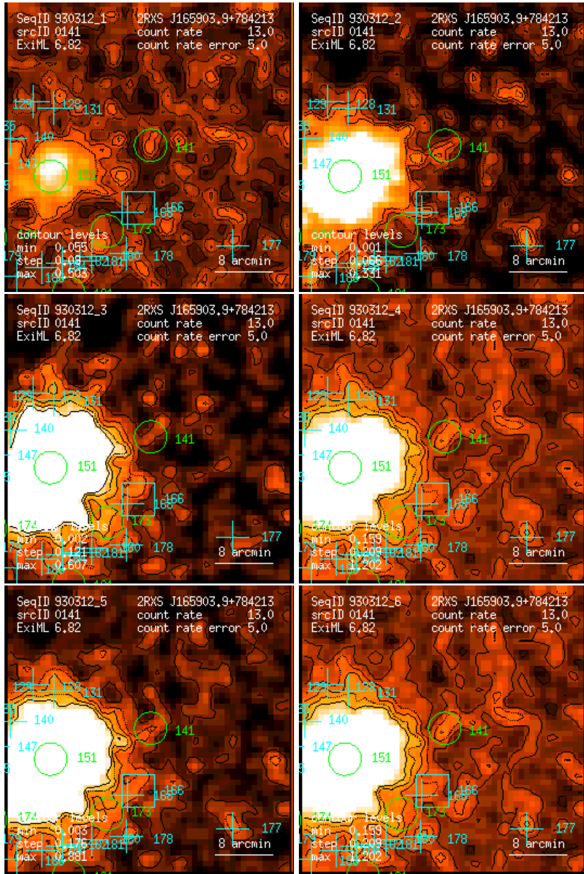
Figure 141: RASS 930312: detection 0141: band rate images, Gaussian filter: (1) PSPC channels 11 – 41, (2) 52 – 90, (3) 91 – 201, (4) 11 – 235, (5) 52 – 201, (6) 11 – 201. Broad band rates in counts/ks. Band rate contour levels in counts/ks/arcmin 2 .
