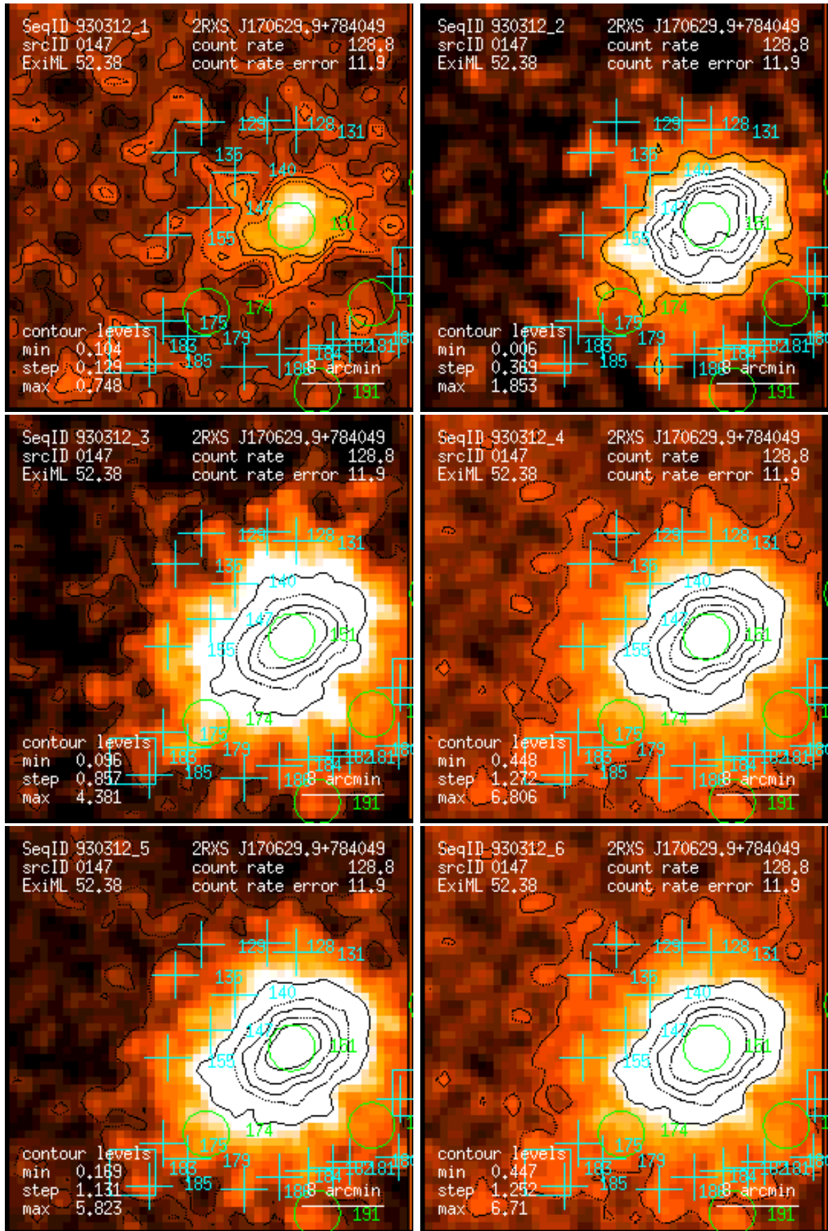
Figure 147: RASS 930312: detection 0147: band rate images, Gaussian filter: (1) PSPC channels 11 – 41, (2) 52 – 90, (3) 91 – 201, (4) 11 – 235, (5) 52 – 201, (6) 11 – 201. Broad band rates in counts/ks. Band rate contour levels in counts/ks/arcmin 2 .
