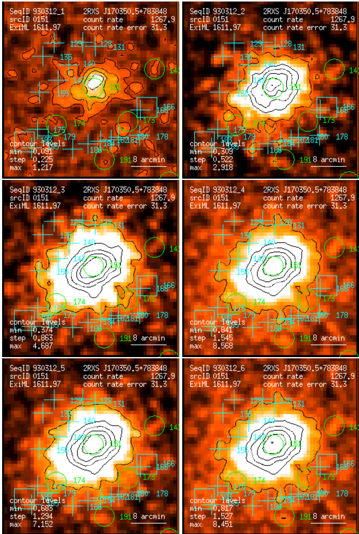
Figure 151: RASS 930312: detection 0151: band rate images, Gaussian filter: (1) PSPC channels 11 – 41, (2) 52 – 90, (3) 91 – 201, (4) 11 – 235, (5) 52 – 201, (6) 11 – 201. Broad band rates in counts/ks. Band rate contour levels in counts/ks/arcmin 2 .
