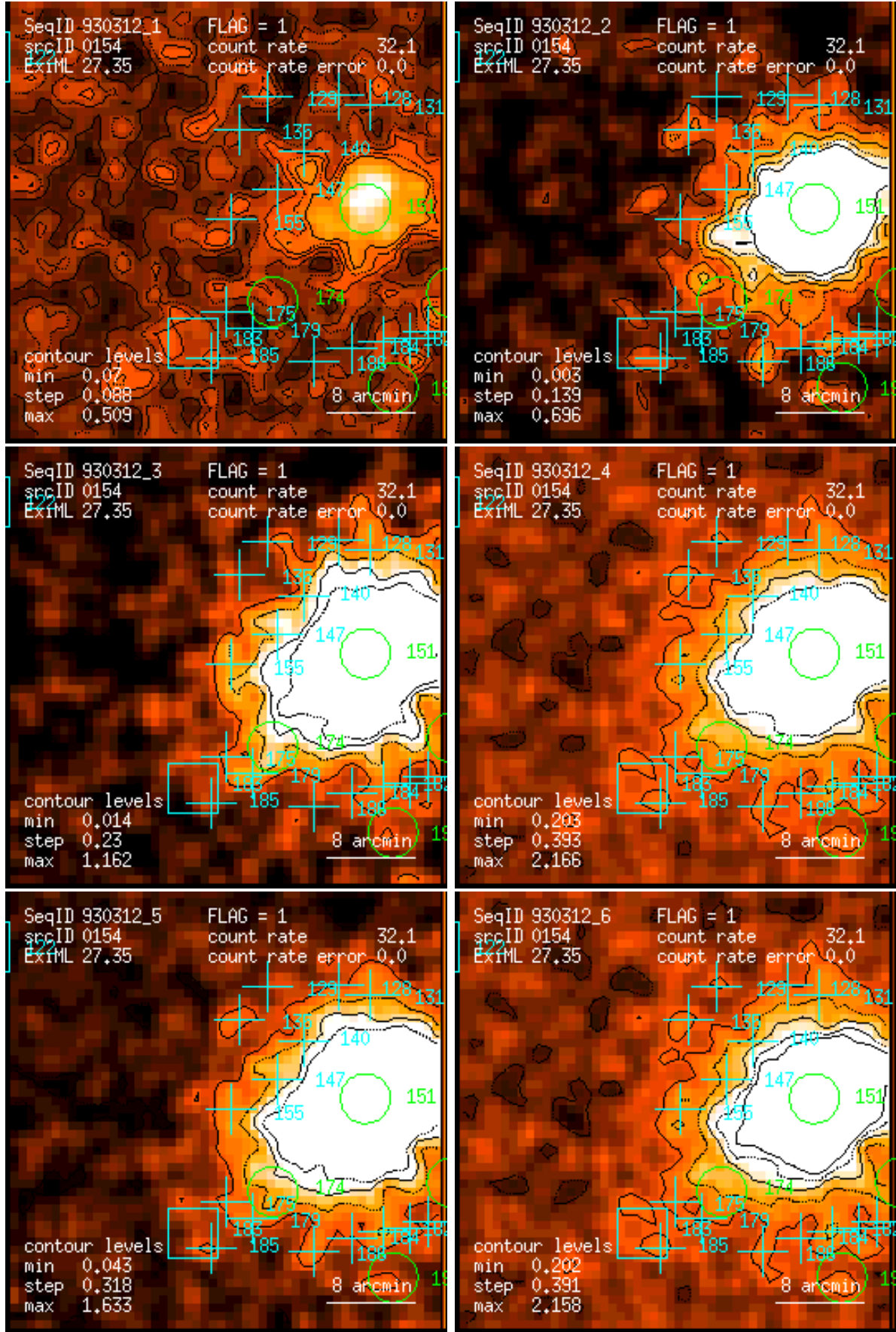
Figure 154: RASS 930312: detection 0154: band rate images, Gaussian filter: (1) PSPC channels 11 – 41, (2) 52 – 90, (3) 91 – 201, (4) 11 – 235, (5) 52 – 201, (6) 11 – 201. Broad band rates in counts/ks. Band rate contour levels in counts/ks/arcmin 2 .
