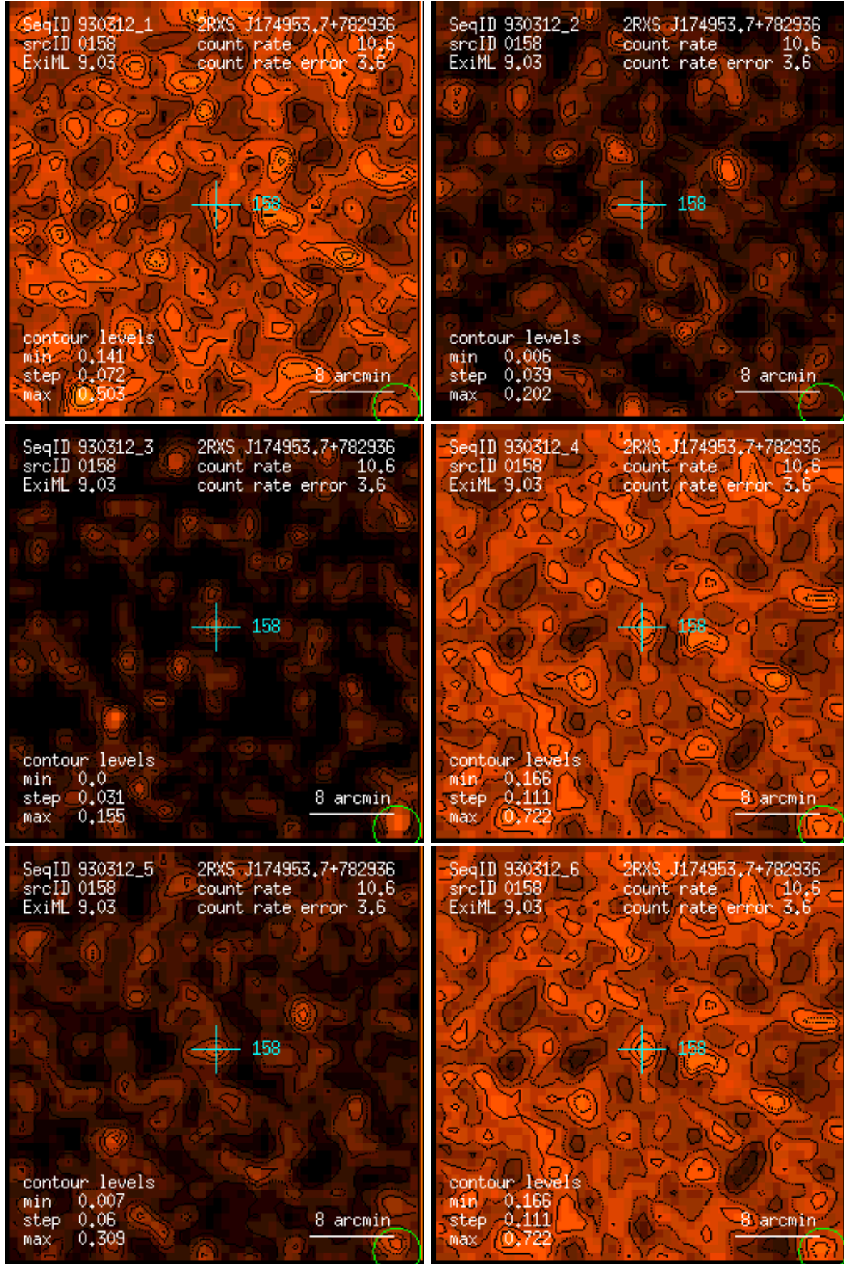
Figure 158: RASS 930312: detection 0158: band rate images, Gaussian filter: (1) PSPC channels 11 – 41, (2) 52 – 90, (3) 91 – 201, (4) 11 – 235, (5) 52 – 201, (6) 11 – 201. Broad band rates in counts/ks. Band rate contour levels in counts/ks/arcmin 2 .
