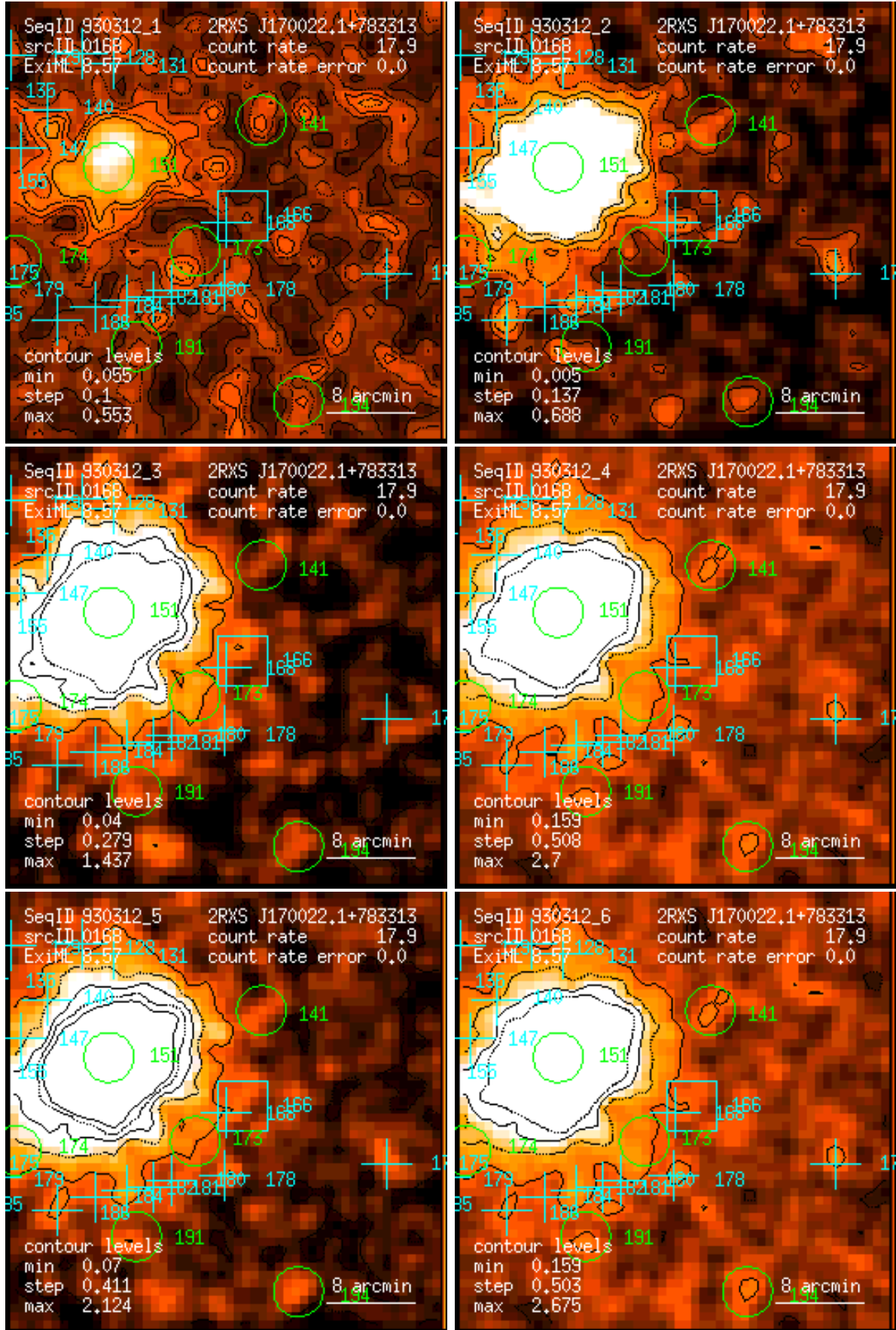
Figure 168: RASS 930312: detection 0168: band rate images, Gaussian filter: (1) PSPC channels 11 – 41, (2) 52 – 90, (3) 91 – 201, (4) 11 – 235, (5) 52 – 201, (6) 11 – 201. Broad band rates in counts/ks. Band rate contour levels in counts/ks/arcmin 2 .
